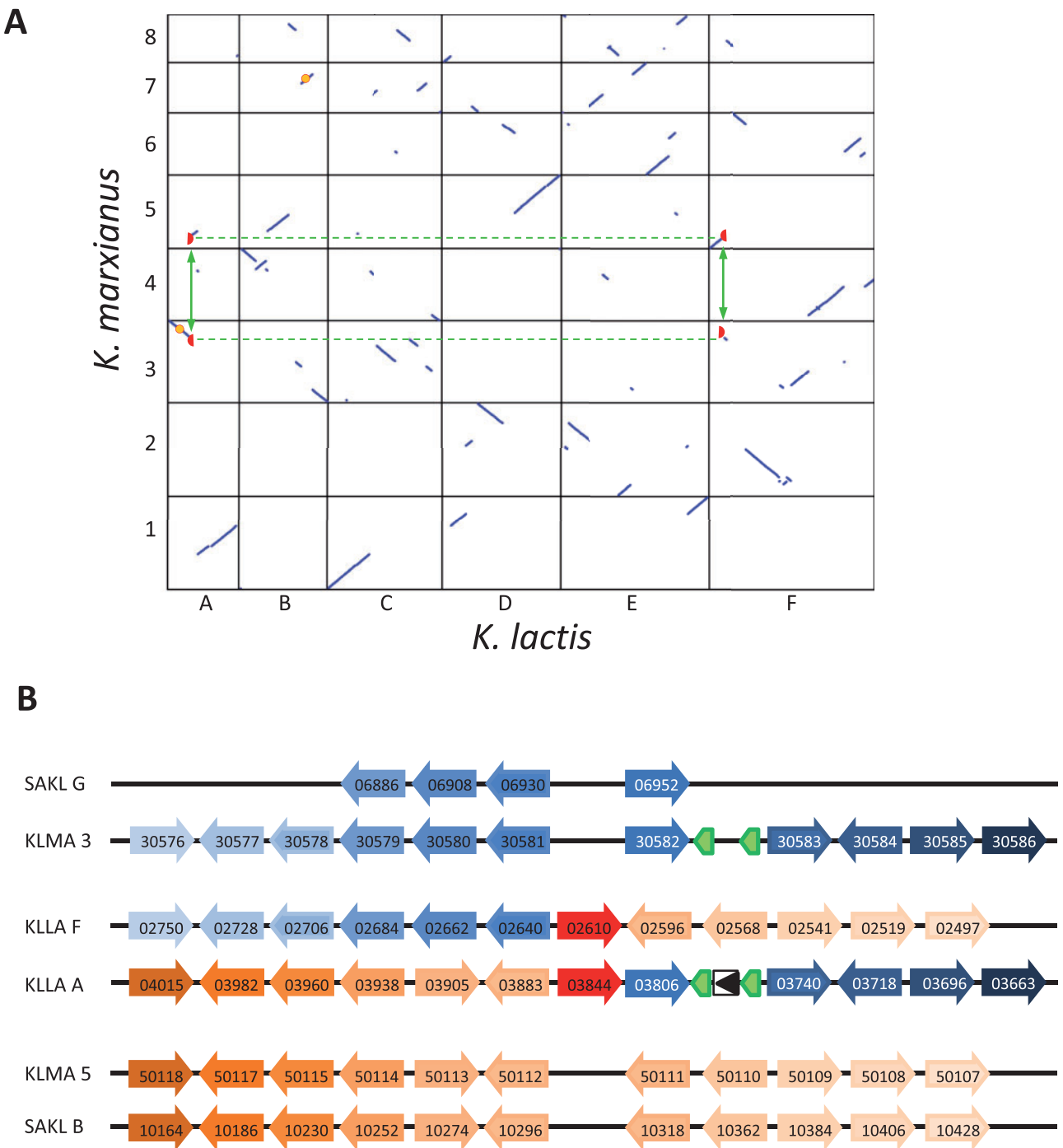
FIG. 8. —Chromosomal rearrangements between Kluyveromyces lactis and Kluyveromyces marxianus . (A) Dotplot of K. lactis and K. marxianus chromosomes, labeled A–F and 1–8, respectively. The two Rover copies found in K. marxianus are depicted as orange disks within a red circle. The two copies of K. lactis elements involved in chromosomal rearrangement are represented by red half-disks. The physical link between the two parts of each K. lactis element is represented by green double arrows and the link between the consecutive chromosomal regions of K. marxianus is represented by green dotted lines. (B) Synteny conservation around the insertion site of K. lactis Rover elements (in red). Chromosome names are on the left and gene names are placed within colored arrows. The Rover element on Klla0F, previously known as KLLA0F02568t and located opposite a CDS of 1,191 amino acids, was reannotated a few kb downstream and now defines a full-length element of 2,458 bp that contains perfect 17-bp TIRs and a degenerate transposase. L. kluyveri orthologous loci on chromosomes G (arrows—blue color gradient) and B (arrows—brown color gradient) were used as outgroups to assess the direction of the reciprocal translocation. Orthologous genes in the three species are represented with the same color. Green arrows correspond to the tRNA genes and the black triangle in KLLA-A corresponds to a single LTR.
