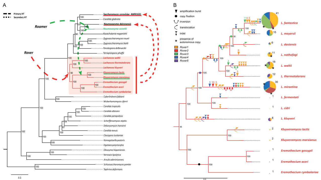
Fig. 1. —Dynamics of Rover and Roamer elements in Ascomycota yeasts. (A) Taxonomic distribution of Rover and Roamer among Ascomycota yeasts suggesting successive HT events. The maximum-likelihood tree was generated from the concatenation of 104 protein sequence alignments. Bootstrap values supporting each clade are indicated on nodes. Rover and Roamer elements were found in the species highlighted in bold. Dotted arrows indicate hypothetical HT events that would explain the patchy distribution of Rover and Roamer elements among Ascomycota. It is hypothesized that a Rover element was initially acquired by the ancestor of the Lachancea/Kluyveromyces/Eremothecium species group—highlighted in red (red dotted line)—and then subsequently diversified in the descendant lineages. Two Rover copies were independently transferred to Saccharomyces cerevisiae strain AWRI1631 and N. dairenensis . Similarly, Roamer seems to have been horizontally transferred to N. castellii (green dotted line), and then further spread to the Kluyveromyces species we studied. (B) Detailed Rover dynamics within the Lachancea/Kluyveromyces/Eremothecium clade. The amplification bursts, the copy fixations, and the chromosomal rearrangements—translocations, inversions, and indels of genes next to a copy insertion site—involving Rover elements are depicted on the maximum-likelihood tree. Amplification bursts are numbered by the count of copies having emerged from the burst according to the transposase phylogeny presented in figure 5. Each event is colored as follows: Orange for Rover1 , red for Rover2 , green for Rover3 , blue for Rover4 , and purple for Rover5 . Genome contents in Rover families are specified by pie charts of a size proportional to the total Rover copy numbers, indicated next to them. Stars notify the presence of autonomous copies from particular families.
