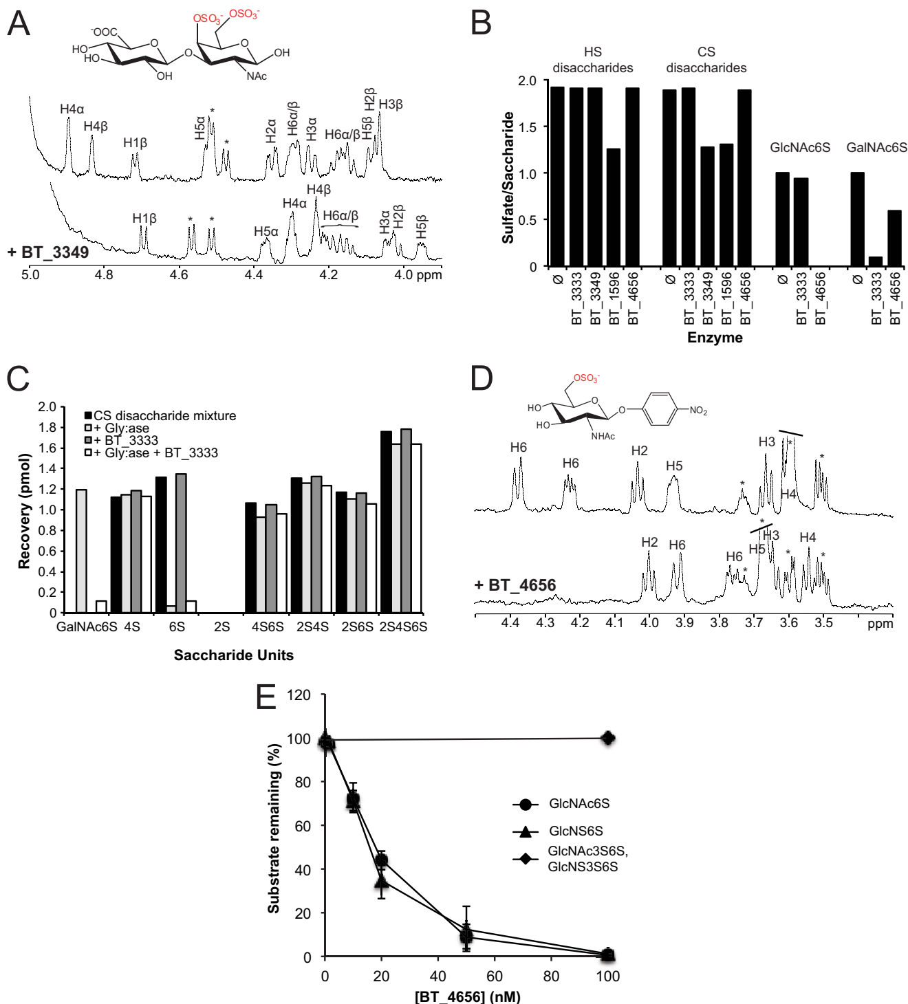
FIGURE 1. Identification of BT_3349 as a 4-O-sulfatase and of BT_4656 and BT_3333 as exosulfatases acting on the 6-O-sulfated nonreducing end hexosamine unit. A, comparison of ^1\text{H} 1D NMR spectra of GlcUA-GalNAc4,6S before (upper trace) and after (lower trace) incubation with BT_3349. The characteristic signals of H4 ( \alpha/\beta ) of GalNAc4,6S at 4.9 and 4.8 ppm are upfield shifted upon incubation with the enzyme. The asterisks denote signals from the glucuronic acid residue. B, mixtures of HS and CS disaccharides were incubated for 1 h at 30 °C with the indicated putative sulfatases. Disaccharides pretreated with glucuronidase to release the nonreducing end \Delta HexA unit were incubated with BT_3333 and BT_4656. All samples were analyzed by RPIP-HPLC and quantified by comparison against known amount of standards. The average number of sulfate groups per unit (either disaccharide mixture or monosaccharide) is indicated for substrates without ( \emptyset ) or with pretreatment by the corresponding enzyme as marked. C, unsaturated CS disaccharide mixture was treated with BT_3333 for 1 h either with or without previous digestion by \Delta 4.5-glycuronidase that converted \Delta 4.5 HexA-GalNAc6S (6S) to GalNAc6S, which was the only structure further digested by BT_3333, whereas all the other unsaturated CS disaccharides present were neither substrates for glucuronidase nor BT_3333. D, ^1\text{H} NMR spectra of GlcNAc6S-O-pNP before (upper trace) and after (lower trace) incubation with BT_4656. Addition of the enzyme results in an upfield shift of the H6 signals indicative of desulfation at position 6 of GlcNAc. The asterisks indicate signals from the buffer. E, to assess the influence of substitution for BT_4656 in either position 3 or position 2, GlcNAc6S, GlcNS6S, N-acetylglucosamine 3,6-O-sulfate, and GlcNS3S6S were incubated at a constant concentration with increasing concentrations of BT_4656 for 1 h, before analysis by RPIP-HPLC. Remaining substrate molecules were quantified as a proportion of originally added monosaccharides.
