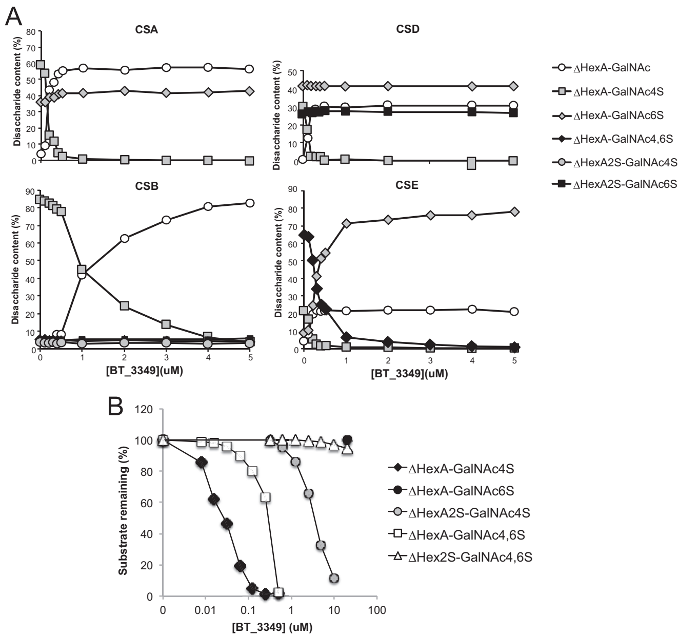
FIGURE 4. Endo-4-O-sulfatase (BT_3349) recognizes 4-O-sulfation in different contexts. A, CS chains A, B, D, and E, as indicated (1 \mu g), were incubated for 8 h with increasing concentrations of enzyme before exhaustive digestion of chains by chondroitinase. Analysis of resulting disaccharides was performed by RPIP-HPLC. Relative proportions of the different disaccharide units recovered were plotted against enzyme concentrations. B, BT_3349 is affected by surrounding sulfation. Constant concentrations of CS-derived disaccharides were incubated for 1 h with increasing concentrations of sulfatase BT_3349 before analysis of products by RPIP-HPLC. Recovered disaccharides were plotted as a proportion of the original starting material.
