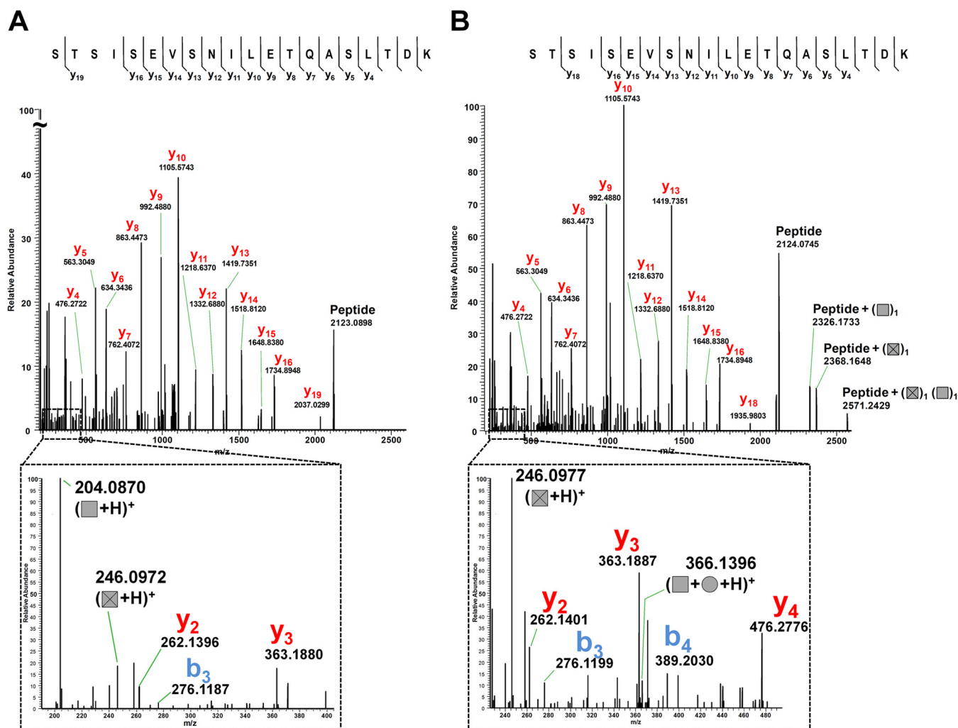
FIG. 6. MS2 spectra of two glycoforms of [192–211] peptide fragmented in HCD illustrating the similar y ion profiles. A, Fragmentation of m/z 925.4455 z = 3 , corresponding to the peptide +1 O-AcHexNAc and +2 HexNAc. B, Fragmentation of m/z 1101.1749 z = 3 , ([192–211] + 1 O-AcHexNAc, 3 HexNAc, 2 Hex). Ions at m/z 204.0872, 246.0977, and m/z 366.1400 are oxonium ions. Glycan symbols: HexNAc (Square), Hex (Circle), O-AcHexNAc (Crossed square).
