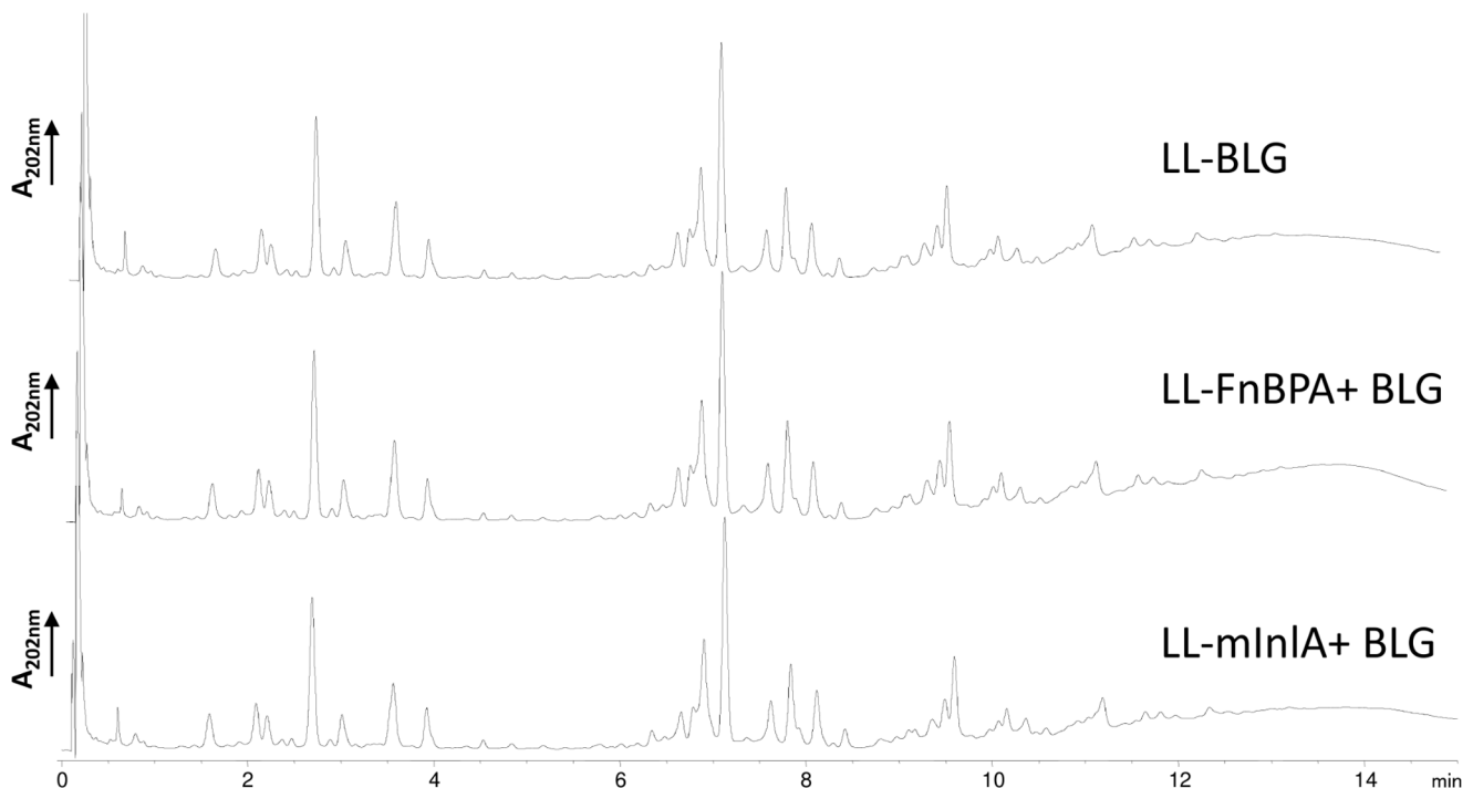
Figure 5. Peptidoglycan composition of cell wall from lactococci recombinant strains. The PG structure of the different strains LL-BLG, LL-FnBPA+ BLG and LL-mInIA+ BLG was compared. PG was extracted from each strain, digested with mutanolysin and the resulting muuropeptides were separated by RP-HPLC. Absorbance was monitored at 220 nm. doi:10.1371/journal.pone.0084509.g005
