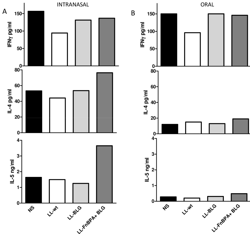
Figure 3. BLG-specific cytokines secreted by BLG-reactivated splenocytes from mice orally or intranasally administered with LL-wt, LL-BLG or LL-FnBPA+ BLG then BLG sensitized. Mice were intranasally (A) or orally (B) administered or not (NS) with LL-wt, LL-BLG or LL-FnBPA+ BLG then sensitized with BLG in Alum. Splenocytes from pooled samples were purified and reactivated with BLG. Secreted cytokines, IFN- \gamma , IL-4 and IL-5 were assayed in medium. The results presented here are from one experiment representative of two performed independently, 8 mice/group. doi:10.1371/journal.pone.0084509.g003
