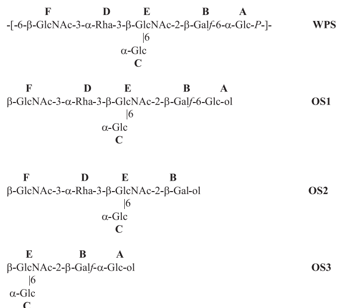
FIGURE 3. Structure of L. lactis MG1363 PS and the oligosaccharide products of its partial hydrolysis (OS1 to OS3). A and C, Glc residues; B, Gal; E and F, GlcNAc, and D, Rha; see also Table 2.
