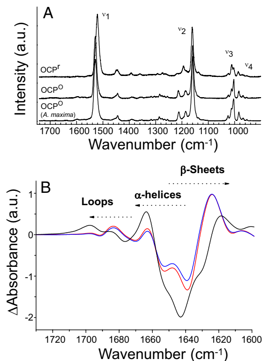
Fig. 4. Changes in the carotenoid and the protein upon illumination. (A) Resonance Raman spectra of Synechocystis PCC 6803 OCP r and OCP o and Arthrospira maxima OCP o in the 1,740 to 820 \text{cm}^{-1} range and (B) light-minus-dark FTIR spectra of OCP in H 2 O (black) and in D 2 O \approx 5 (red line) and 50 (blue line) seconds after illumination with a blue LED in the carbonyl region between 1,730 and 1,600 \text{cm}^{-1} (Amide I region). The OCP r minus OCP o Amide I differential pattern is assigned to H-bond loosening (upshift) of the loops and \alpha -helices carbonyl modes together with a H-bond strengthening (downshift of carbonyl modes) of the \beta -sheet.
