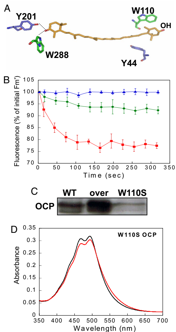
Fig. 3. The OCP r is essential for the induction of the photoprotective mechanism. (A) Shown is 100% conserved Tyr and Trp interacting with the carotenoid. (B) Decrease of Fm' during exposure of WT (red squares), overexpressing W110S OCP mutant (green circles), and His-tagged W110S OCP resistant mutant (blue triangles) cells to 740- \mu\text{mol photons m}^{-2} \text{s}^{-1} of blue-green light (400–550 nm). (C) Immunoblot detection in membrane-phycobilisome fractions from WT (1), overexpressing W110S OCP mutant (2), and His-tagged W110S OCP (3). Each lane contained 1.5- \mu\text{g} chlorophyll (D). Absorbance spectra of the dark orange form (OCP o ; black) and the light form (OCP r ; red). The OCP o was illuminated during 15 min at 1,200- \mu\text{mol photons m}^{-2} \text{s}^{-1} and at 10°C.
