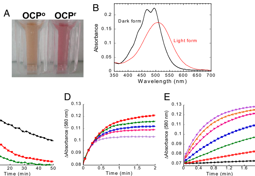
Fig. 2. Isolated OCP is responsive to blue-green light: Photoconversion and dark recovery. (A) Photograph of isolated OCP o and OCP r . To obtain OCP r the isolated protein was illuminated with a blue-green light at 740- \mu\text{mol photons m}^{-2} \text{s}^{-1} at 12°C for 2 min. (B) Absorbance spectra of the dark orange form (OCP o ; black) and the light red form (OCP r ; red). (C) Darkness red OCP r to orange OCP o conversion (decrease of the absorbance at 580 nm) and (D) photoconversion from the OCP o to the OCP r form using a 350- \mu\text{mol photon m}^{-2} \text{s}^{-1} blue-green light intensity (increase of the absorbance at 580 nm) at different temperatures: 32°C (violet), 28°C (rose), 24°C (blue), 19°C (green), 15°C (red), and 11°C (black). (E) OCP r accumulation at 11°C and different light intensities: 20 (black), 50 (red), 120 (green), 210 (blue), 350 (rose), 740 (orange), and 1,200 (violet)- \mu\text{mol photons m}^{-2} \text{s}^{-1} of blue-green (400–550 nm). The protein concentration was OD 0.2 at 495 nm.
