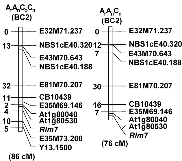
Supplemental Figure 3: Maps of the A7 linkage group in BC2 progenies of the allotriploid (ArAnCn) and allotetraploid (ArAnCoCn) hybrids.
