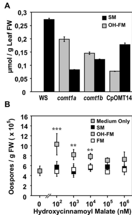
Figure 5. 2-O-5-hydroxyferuloyl-L-malate accumulates in comt1 mutants, and promotes oomycete sexual reproduction in vitro . (A) Quantification of sinapoyl malate (SM) and 5-hydroxyferuloyl malate (OH-FM) in methanolic extracts of 4 week-old plantlets from the different A. thaliana lines. The compounds were quantified by HPLC referring to synthetic standards. The bars represent mean values \pm SD from 3 experiments. (B) Effect of different concentrations of SM, OH-FM, and feruloyl malate (FM) on sexual reproduction of Phytophthora cactorum isolate 723 in vitro . Displayed are means \pm SD from 4 repetitions. Statistically significant differences for OH-FM values compared with values in the absence of the compound were determined by Student's t-test (** P < 0.001 , *** P < 0.0001 ). FW = fresh weight. doi:10.1371/journal.ppat.1000264.g005
