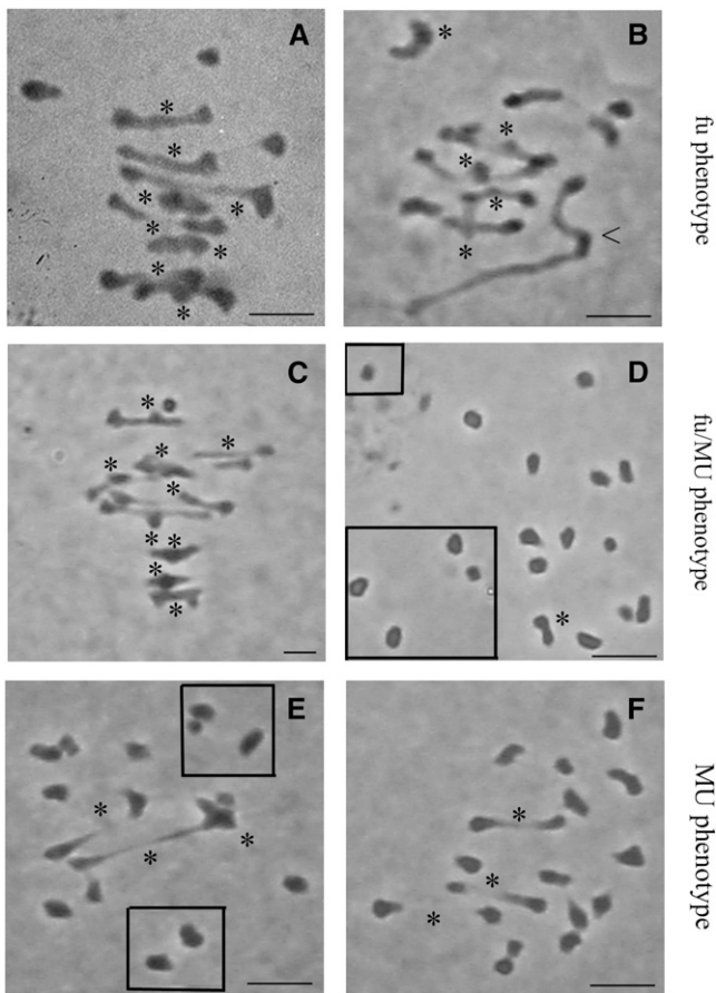
Figure 1. Representative MI Nuclei of B. napus Allohaploids Showing Contrasting Meiotic Behaviors.
