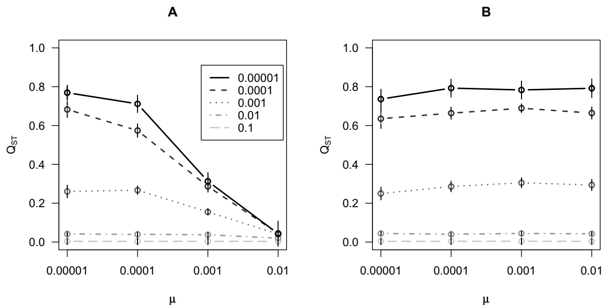
Figure 3 Results for computer simulations for Q_{ST} . The effect of mutation rate and migration rate on Q_{ST} . Different lines represent different migration rates. Migration rates 0.1, 0.01, 0.001, 0.0001 and 0.00001 correspond to different lines as indicated by the legend in panel A. Points are means of 50 replicate simulations and vertical lines correspond to 95% confidence intervals. In panel A) results for the random mutation model, panel B) results for the incremental mutation model.
