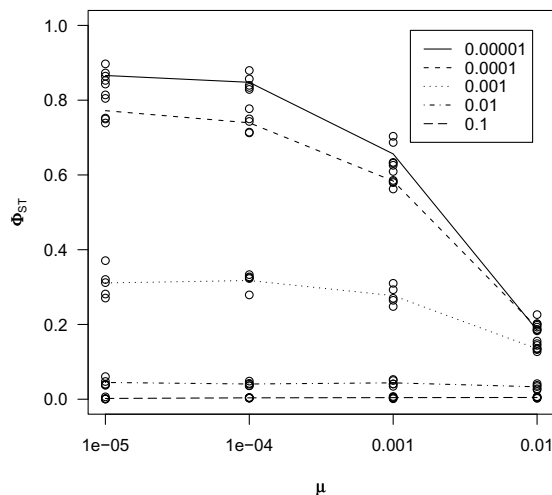
Figure 2 Results of computer simulations for mixed mutation model. The effect of mutation rate on genetic differentiation calculated from \Phi_{ST} using mixed mutation model. In this model, there was a probability of 0.2 that when a mutation occurs the allele will mutate to any state. Different lines represent different migration rates. Migration rates 0.1, 0.01, 0.001, 0.0001 and 0.00001 correspond to different lines as indicated by the legend.
