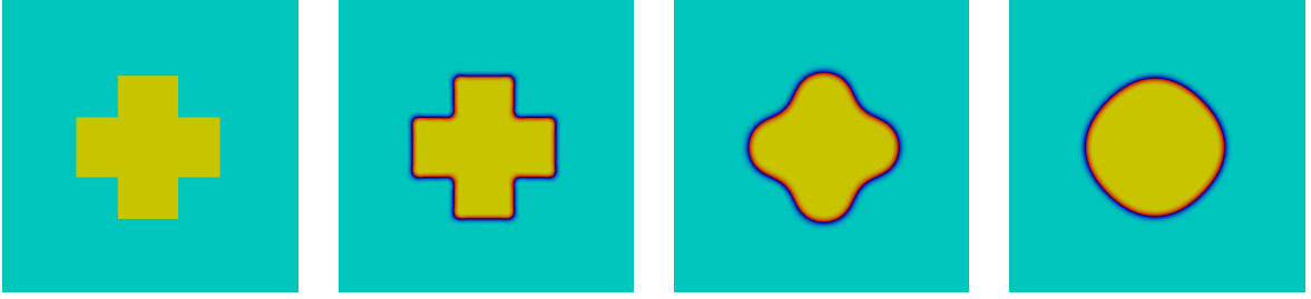
Figure 5: Evolution of a cross-shaped interface. Displayed times are 0 , 5 \cdot 10^{-5} , 1 \cdot 10^{-2} , 8.17 \cdot 10^{-2} .
