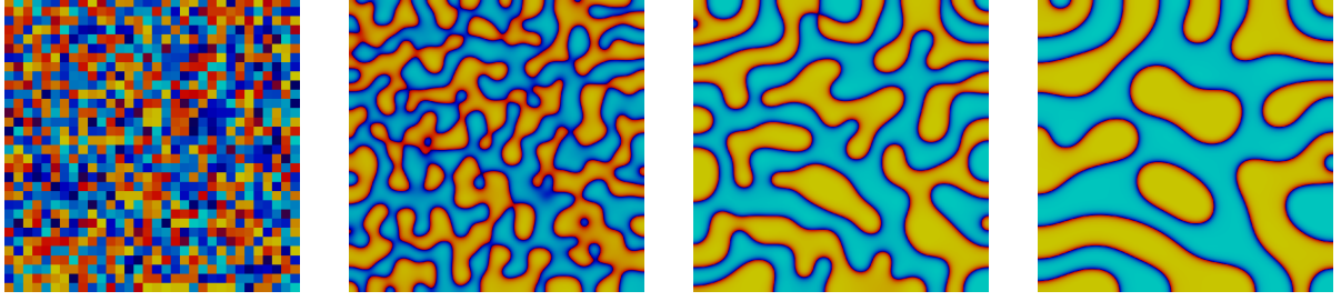
(a) 128 \times 128 uniform Cartesian mesh, k = 0 , BE
