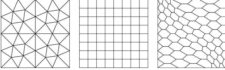
Figure 1: Mesh families for the numerical tests
