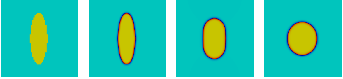
Figure 4: Evolution of an elliptic interface. Displayed times are 0 , 3 \cdot 10^{-3} , 0.3 , 1 .
