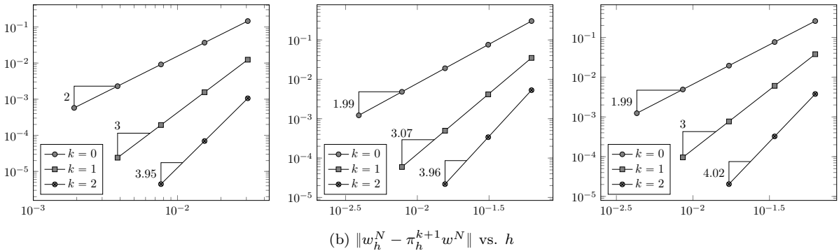
Figure 3: L^2 -errors at final time vs. h . From left to right: triangular, Cartesian and (predominantly) hexagonal mesh families; cf. Figure 1.
