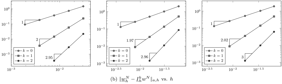
Figure 2: Energy-errors at final time vs. h . From left to right: triangular, Cartesian and (predominantly) hexagonal mesh families; cf. Figure 1.
