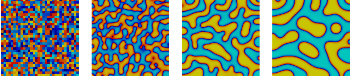
(b) 64 \times 64 uniform Cartesian mesh, k = 1 , BDF2
