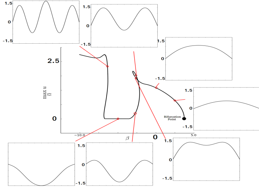
Figure 4: Bifurcation branch from \bar{\beta} = \frac{1-\lambda_1^2}{\lambda_1} with \Omega = (0, 2\pi) and some sols. to (1.1). Along the branch the positivity is lost and even negative solutions appear. Here the branch does not return to the region \beta > 0 since the complexity of solutions is constrained by |\Omega| . Indeed, |u| < \sqrt{2} for \beta > 0 (see the introduction) implies \int_{\Omega} (u'')^2 + \beta(u')^2 dx = \int_{\Omega} u^2 - u^4 dx \leq 6|\Omega| .
