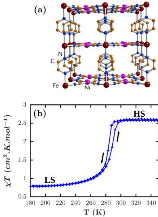
FIG. 1. (Color online) (a) Perspective view of the structure of the [Fe(pyrazine)(Ni(CN) 4 )] complex and (b) the product of the magnetic susceptibility and the temperature as a function of the temperature in the heating and cooling modes for 50 nm [Fe(pyrazine)(Ni(CN) 4 )] particles.
