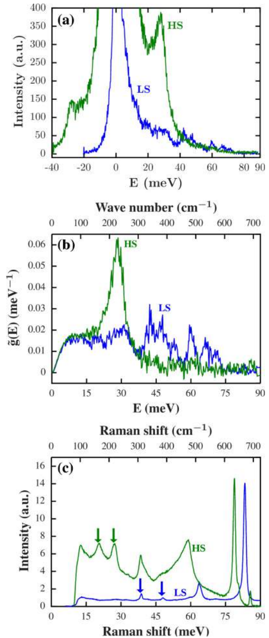
FIG. 2. (Color online) NIS spectra (a), iron-DOS (b), and Raman spectra (c) of 50-nm [Fe(pyrazine)(Ni(CN) 4 )] nanoparticles in the two spin states. The central peak of (a) is the elastic absorption, while the peaks on the right and on the left are the Stokes (phonon creation) and the anti-Stokes (phonon annihilation) peaks respectively. Their ratio depends on the temperature. Thereby, in the LS state, the anti-Stokes peaks have a very low intensity when compared to the Stokes peak. In (c), the arrows show, from the left to the right, the \nu(\text{FeN}_{\text{cycle}}) and the \nu(\text{FeN}_{\text{NC}}) modes in the two spin states.
