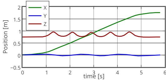
Fig. 7: Experiment 3: COM trajectory for the running scenario. One can recognize the ballistic shape of the Z component.
