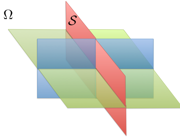
FIGURE 3. Internal corner : \{x_1 x_2 x_3 = 0\}
