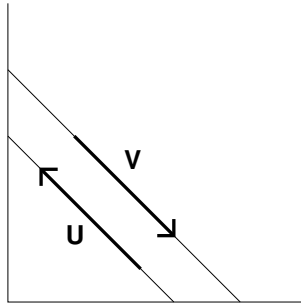
FIGURE 9. The case \mathbf{U} = -\mathbf{V} .
