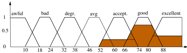
Fig. 4: QUALITY defuzzification
