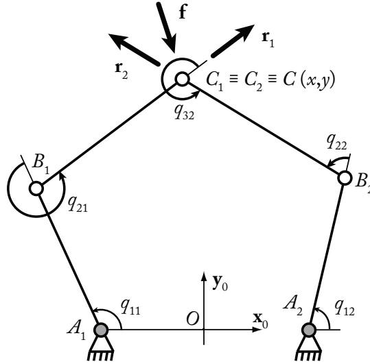
Fig. 4 Kinematic chain of the five-bar mechanism
