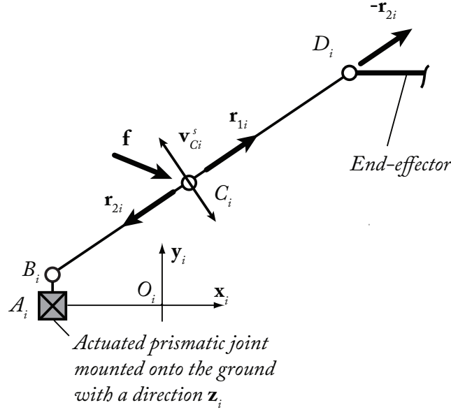
Fig. 7 Leg i of the Tripteron in a LPJTS singularity
