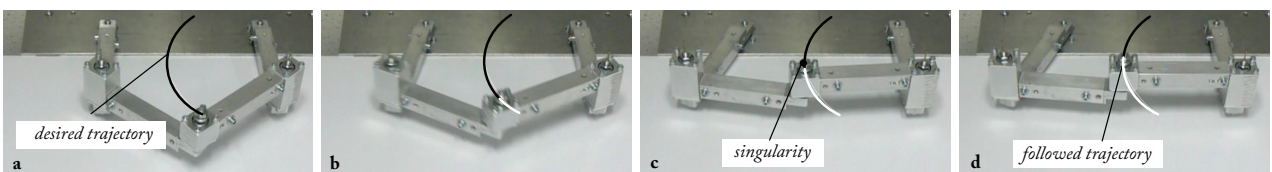
Fig. 22 The five-bar mechanism tracking the trajectory which does not respect the dynamic criterion (65)
