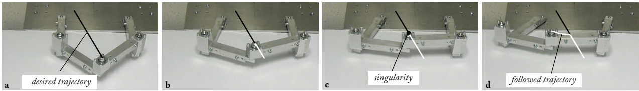
Fig. 13 The five-bar mechanism tracking the trajectory which does not respect the dynamic criterion (62)
