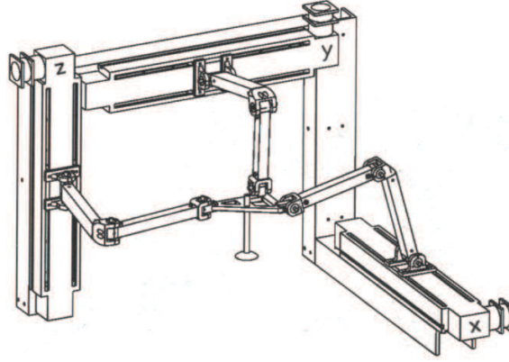
(a) CAD view (courtesy of C.M. Gosselin)
