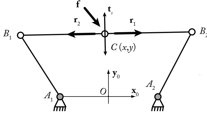
Fig. 5 The five-bar mechanism in a Type 2 singularity: the uncontrollable motion is described by the vector \mathbf{t}_s
