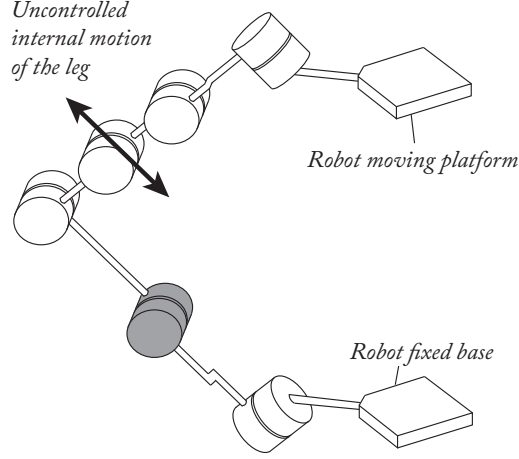
Fig. 3 Example of LPJTS singularity for a parallel robot leg (grey joints denote actuated joints): in that case, for a fixed position of the end-effector, the leg gains one instantaneous uncontrollable motion due to the particular arrangement of the passive joints
