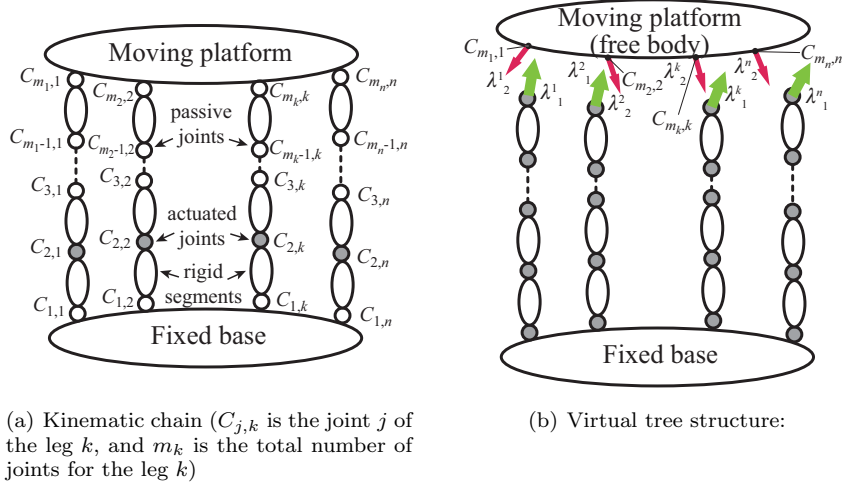
Fig. 1 A general parallel robot (grey circles denote actuated joints).
