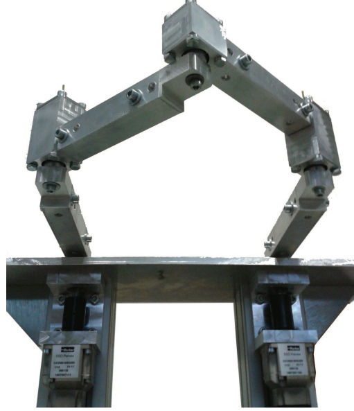
Fig. 8 Five-bar mechanism designed and manufactured at IFMA
