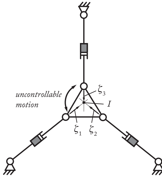
Fig. 2 Example of Type 2 singularity of a 3- RPR planar parallel robot (grey joints denote actuated joints): in that case, the platform has one uncontrollable motion which is an instantaneous rotation around the point I
