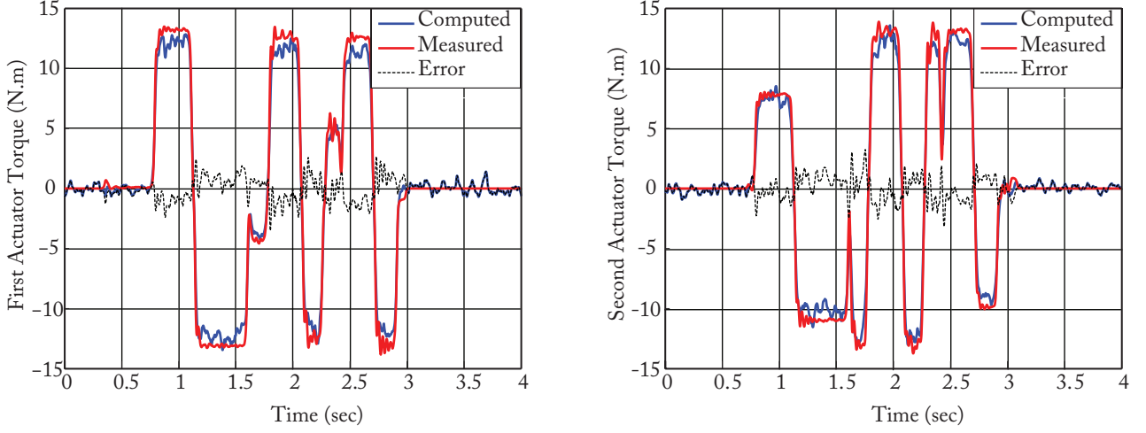
Fig. 9 Verification of the identified dynamic model
