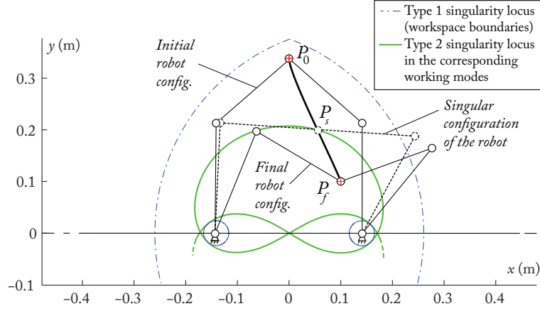
Fig. 10 Starting point P_0 and ending point P_f of the Type 2 singularity crossing trajectory
