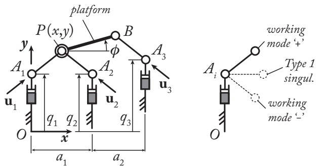
(a) Kinematic architecture of the robot
