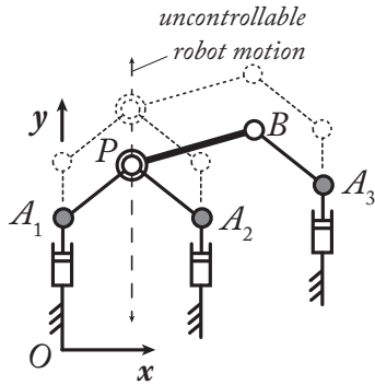
(a) When all leg directions \underline{u}_i are observed (Case 1): a 3- \underline{PRR} robot
