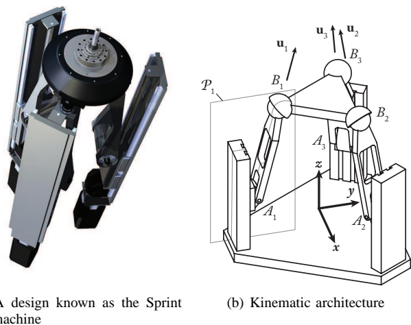
Fig. 20. The spatial 3- PRS robot with parallel P joints.
