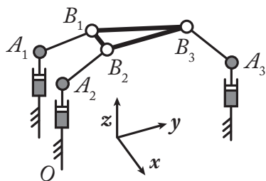
(c) When all leg directions \underline{u}_i and the Plücker coordinates of the lines passing through the legs 1 and 3 are observed (Case 3): a 3- PRS robot
