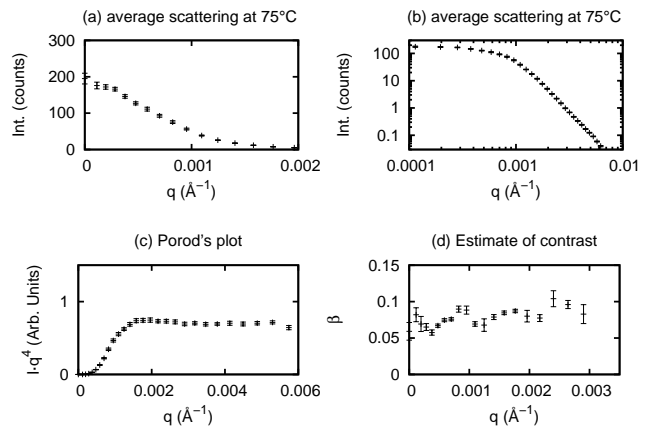
FIG. 5. Circular average of the intensity of Fig. 4. The isotropic intensity corresponds to sets of 50 frames of 1s (a and b). We plot the number of counts per pixel in 50 s (filters were set) and we estimate a domain size of \simeq 0.15 \mu . “Porod’s” plot (c) shows a q^{-4} asymptotic behaviour. This behaviour proves that well defined domains are present, separated by antiphase walls. The speckle contrast \beta (d) is defined in Eq. 3. We estimate \beta \simeq 7.5\% . Our total measurement of 300 frames was split in 6 sets of 50 frames for the estimate of averages and errors.
