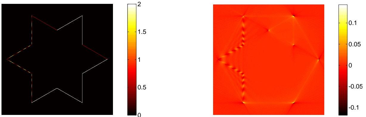
FIGURE 2. The object f is on the left and FBP of the resulting reflective sinogram is on the right.
