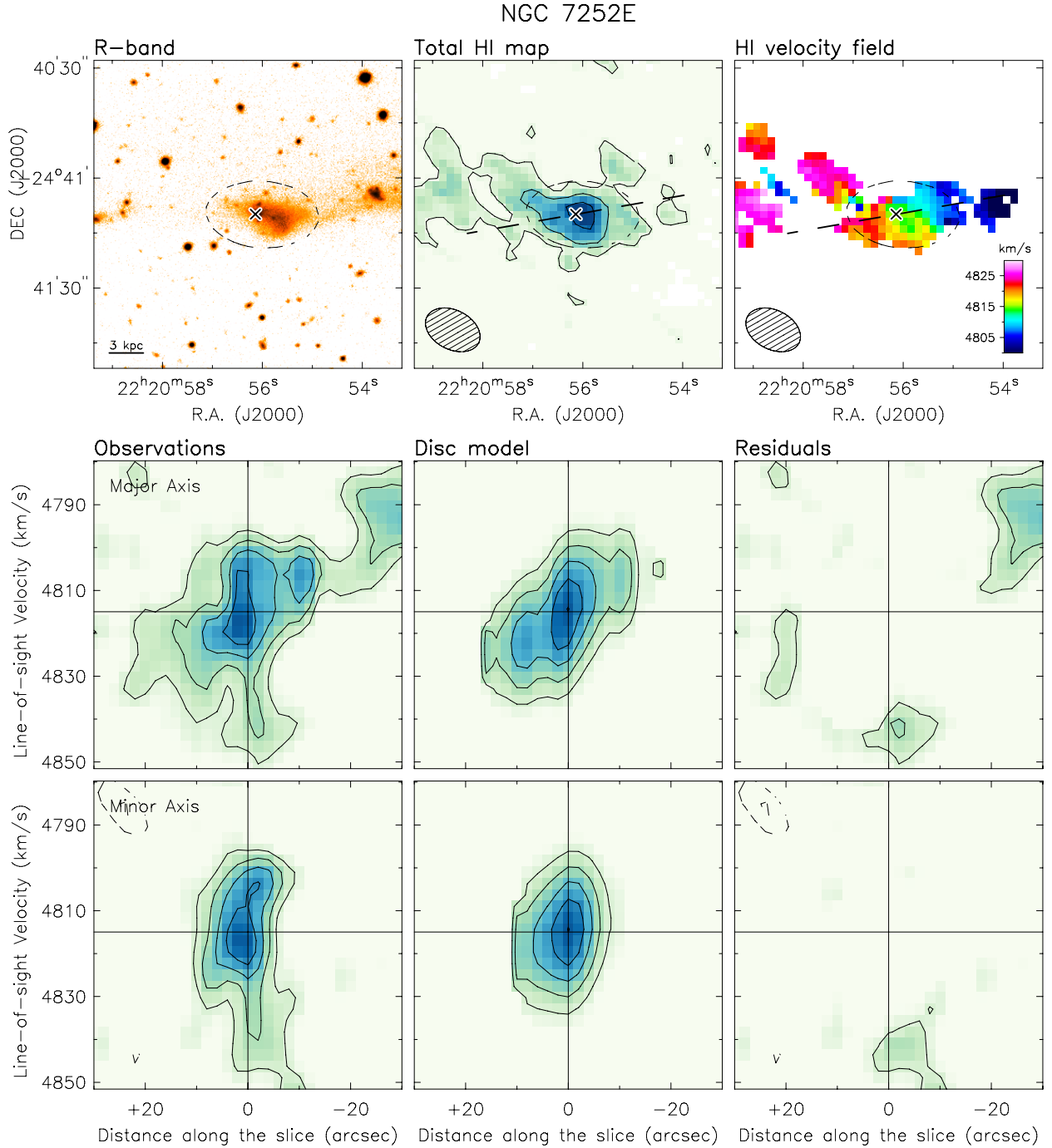
Fig. 8. Same as Fig. 5 for NGC 7252E. In the total HI map, contours are at \sim 1.5, 3.0, \text{ and } 4.5 M_{\odot} \text{ pc}^{-2} .
