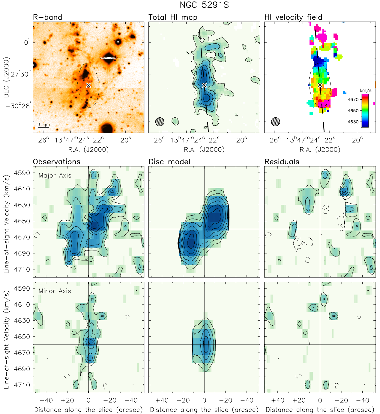
Fig. 6. Same as Fig. 5 for NGC 5291S. In the total HI map, contours are at \sim 4.5, 9, 13.5, 18 M_{\odot} \text{pc}^{-2} .
