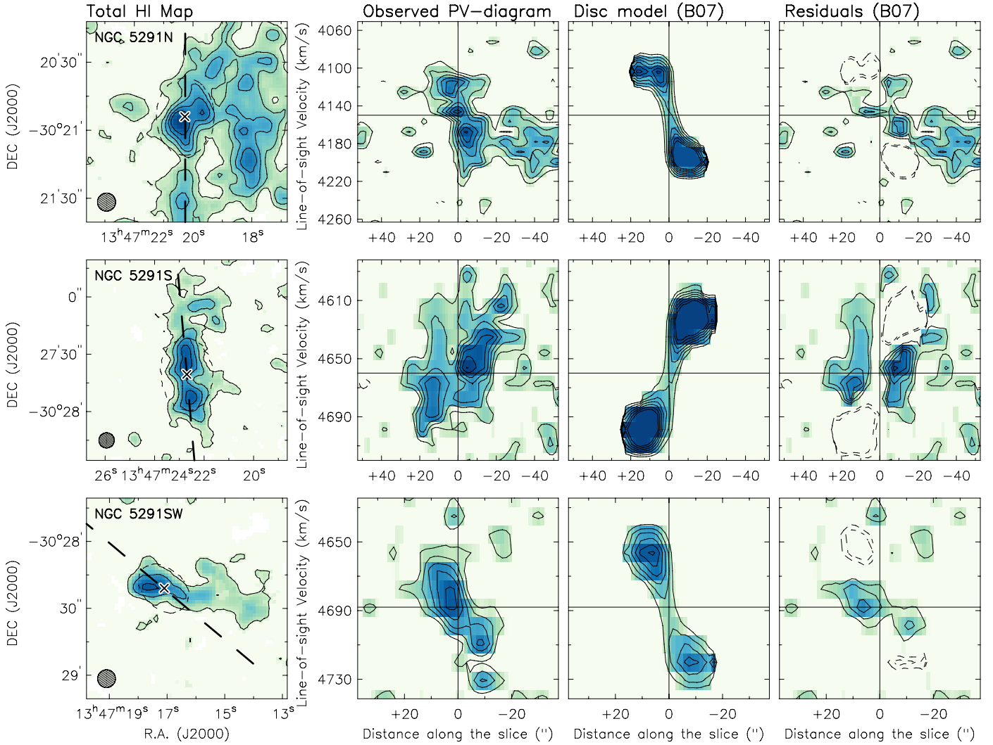
Fig. B.1. Disc models for NGC 5291N ( top ), NGC 5291S ( middle ), and NGC 5291SW ( bottom ) adopting the parameters from B07. Left panels: total HI maps from the observed cube (solid contours) and the model cube (dashed ellipse). The cross and dashed line illustrate the kinematical centre and major axis, respectively. The circle and the bottom-left corner shows the HI beam. Right panels: PV diagrams along the major axis obtained from the observed cube, model cube, and residual cube. Solid contours range from 2\sigma to 8\sigma in steps of 1\sigma . Dashed contours range from -2\sigma to -4\sigma in steps of -1\sigma . The horizontal and vertical lines correspond to the systemic velocity and dynamical centre, respectively.
