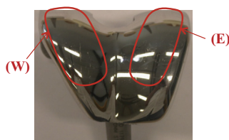
Fig. 1. The 2 wear zones of analysis.
