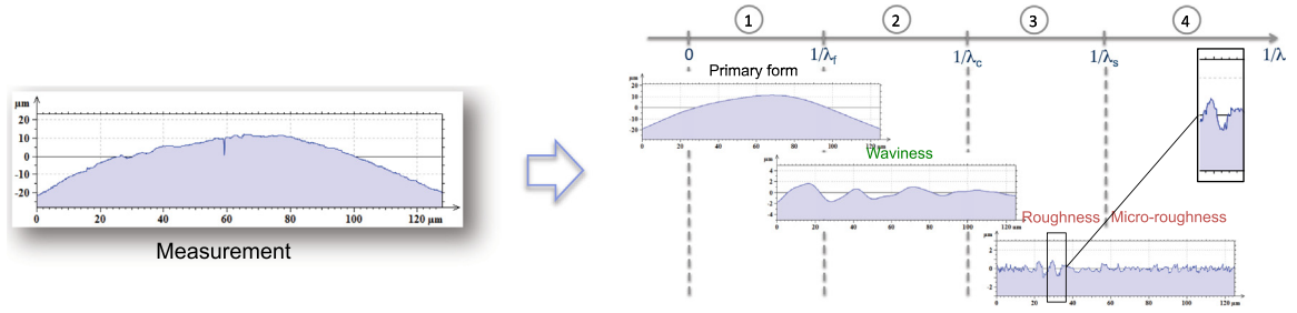
Fig. 2. Separation of roughness, waviness and primary form.
