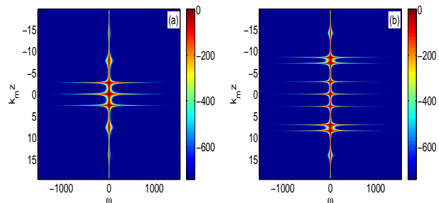
FIG. 7. (Color online) The spectrum of the generalized Peregrine soliton log scale, i.e. \log |F(\omega, z)| with A=1 . (a) d_m = 5 , (b) d_m = 10 .
