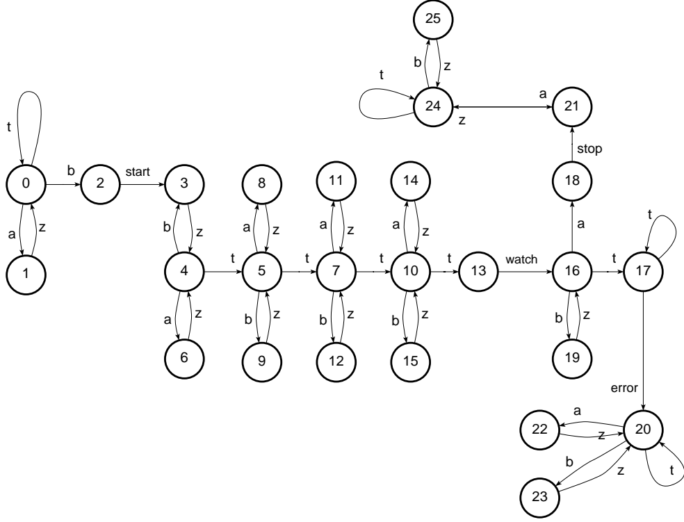
Figure 3: State graph for (Universal || Present)
