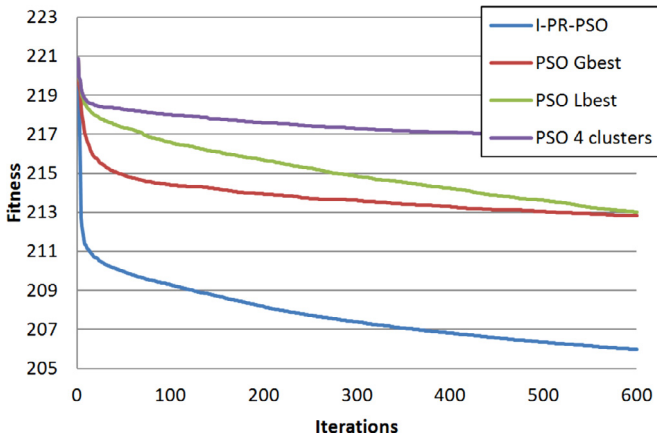
Fig. 20. Shifted Ackley.
