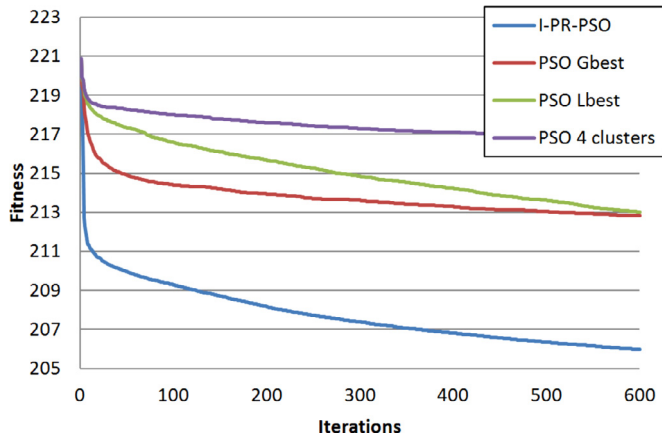
Fig. 20. Shifted Ackley.
