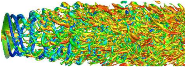
Figure 14: J = 0.20 - Instantaneous vortical structures visualization ( \lambda_2 = -2 ).
