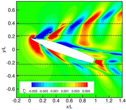
(c) URANS k-\omega SST 27M
