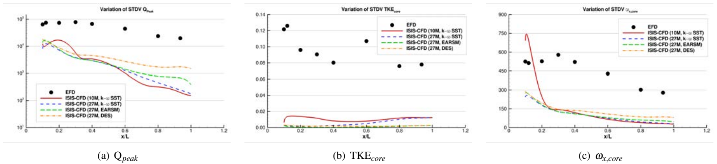
FIGURE 10. EFD AND CFD VARIABLES IN SDTV CORE VORTEX
