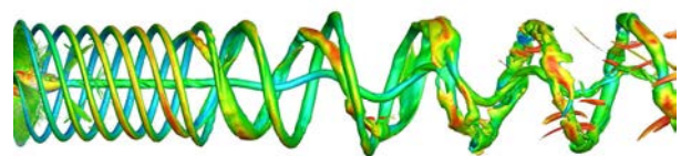
Figure 9: J = 0.71 - Y-component of vorticity (upper half) and turbulence kinetic energy (lower half).
