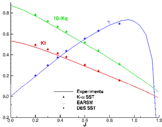
Figure 6: Open-water characteristics of the E779A propeller.
