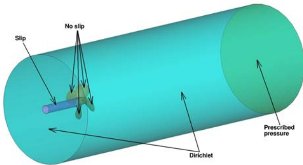
Figure 3: Computational domain with the boundary conditions.
