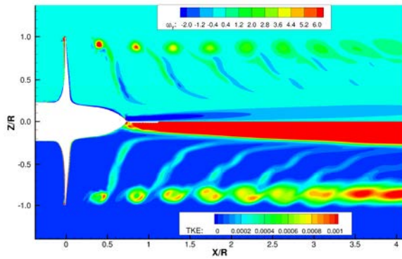
(a) k- \omega SST
