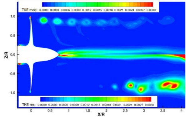
Figure 13: J = 0.45 - Modelled turbulence kinetic energy (upper half) and resolved turbulence kinetic energy (lower half).
