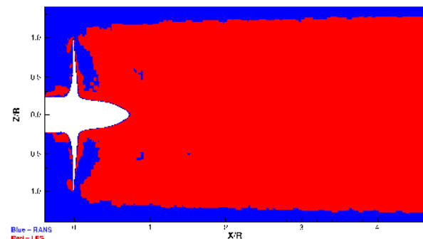
Figure 8: J = 0.71 - Visualisation of the DES function (red: LES region, blue: RANS region).
