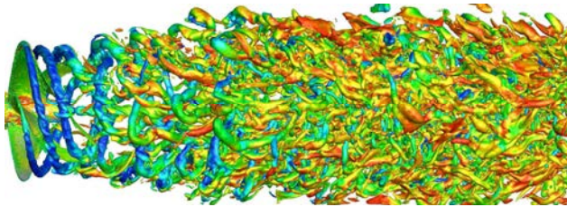
Figure 14: J = 0.20 - Instantaneous vortical structures visualization ( \lambda_2 = -2 ).
