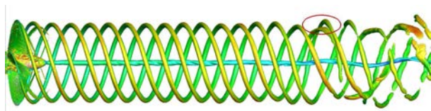
Figure 10: J = 0.71 - Instantaneous visualization of the vortical structures ( \lambda_2 = -2 ).
