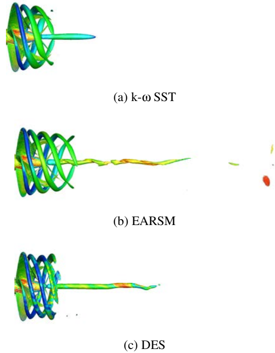
Figure 14: J = 0.20 - Vortical structures visualisations ( \lambda_2 = -2 ).
