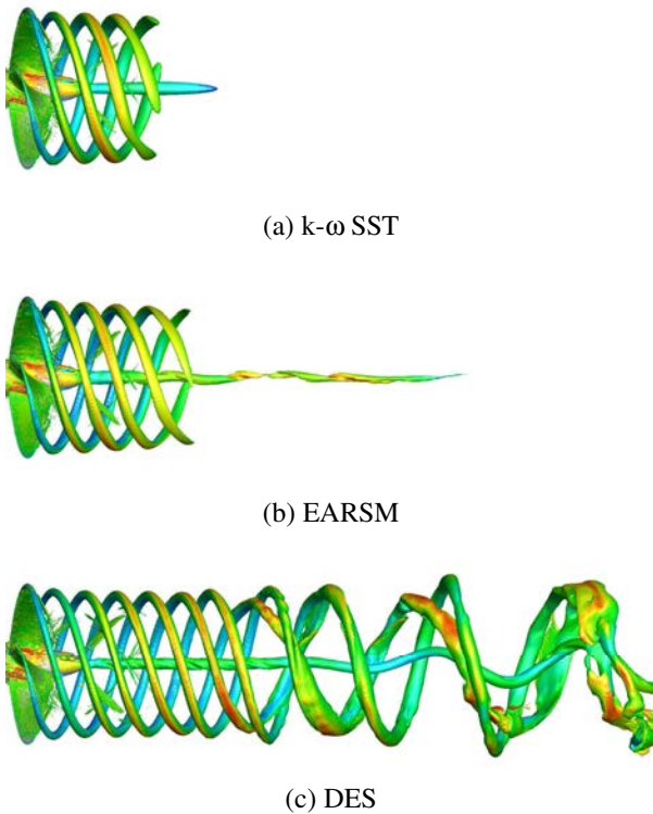
Figure 12: J = 0.45 - Vortical structures visualisations ( \lambda_2 = -2 ).
