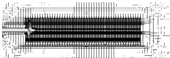
Figure 4: View of the mesh in the symmetry plane
