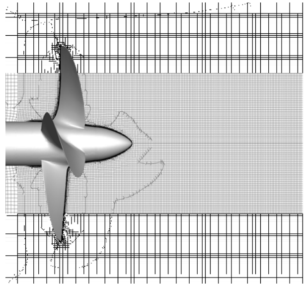
Figure 5: View of the mesh detail in the symmetry plane.
