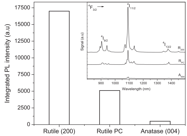
Fig. 10. UV excited room temperature integrated luminescence of 1% \text{Nd}^{3+} doped R_{200} , R_{PC} and A_{004} samples. Characteristics \text{Nd}^{3+} 4F_{3/2} \rightarrow 4I_J transitions obtained in each \text{TiO}_2 film are represented in insert.
