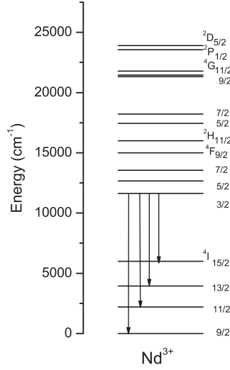
Fig. 4. Energy diagram of Nd 3+ ion [26].
