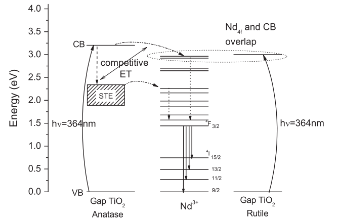
Fig. 8. Energy transfer mechanism describing competitive transfer and Nd 3+ sensitisation in A-TiO 2 and R-TiO 2 . One UV-blue photon absorbed by a Nd 3+ ion is converted to one Nd 3+ NIR photons through a two-step sequential energy transfer. Solid, curved dotted, and straight arrows represent optical transition, non-radiative energy transfer, and non-radiative relaxation.
