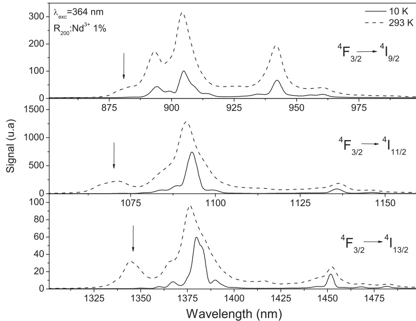
Fig. 5. 10 K and room temperature PL of 1% Nd 3+ -doped R 200 film.
