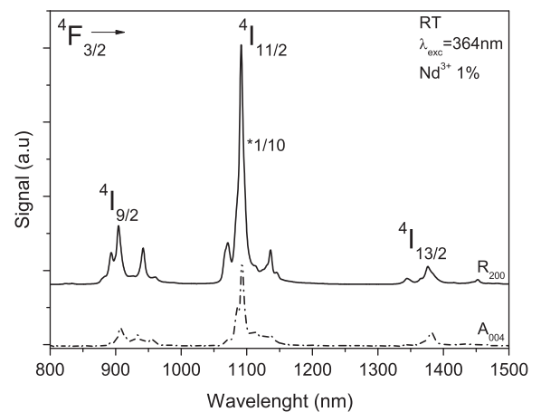
Fig. 3. Room temperature emission spectra under excitation at 364 nm of 1% Nd 3+ -doped anatase and rutile thin films. The real intensity of PL spectrum of Nd 3+ -doped R 200 is 10 times greater.
