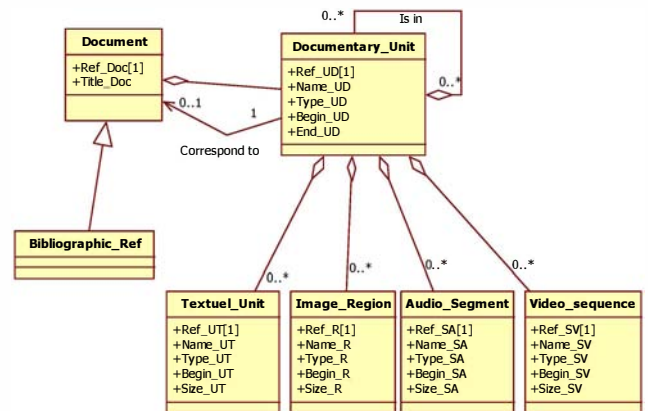
Figure 5. Meta-model of documents
