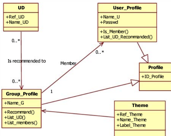
Figure 6. Canonical model of user profile management recommendations
