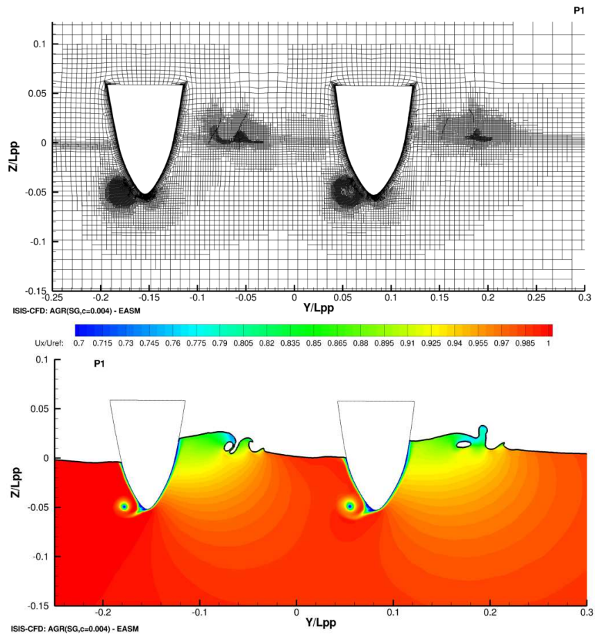
Figure 1: Flow around a catamaran in sideways motion: transverse cuts show the two hulls, the refined mesh (top), the axial velocity with longitudinal vortices and breaking bow waves (bottom).
