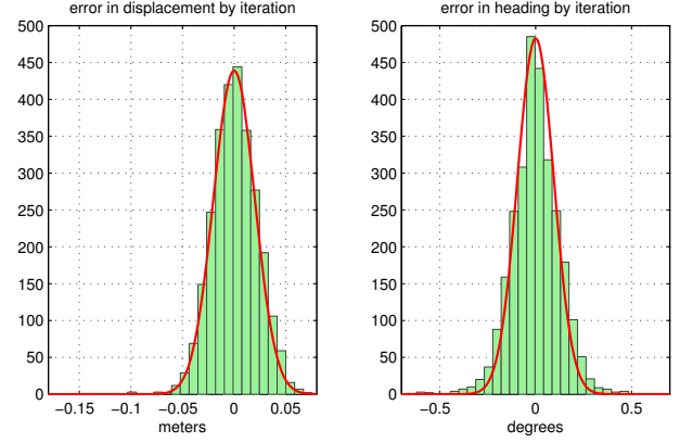
Fig. 6. Errors in heading and displacement by iteration during the test.
