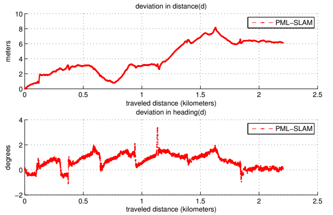
Fig. 7. Deviation from real path in distance and heading along journey.
