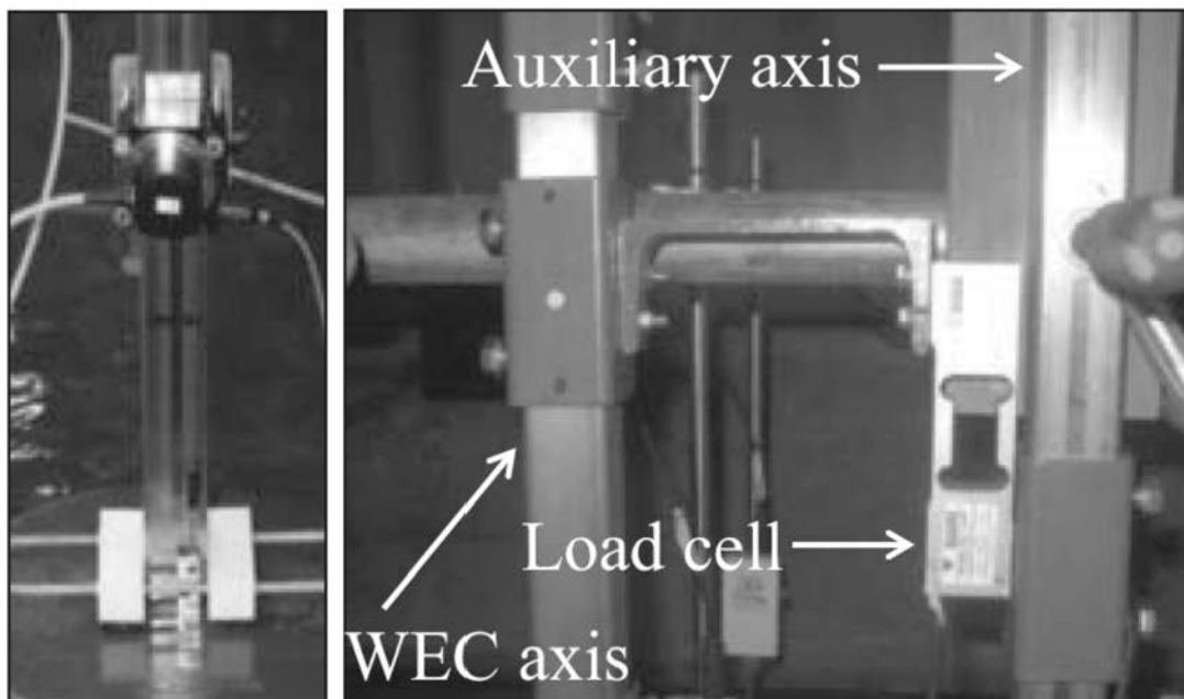
Figure 8: Rotary potentiometer (left); Load cell (right), both installed at the top of the WEC axis.
