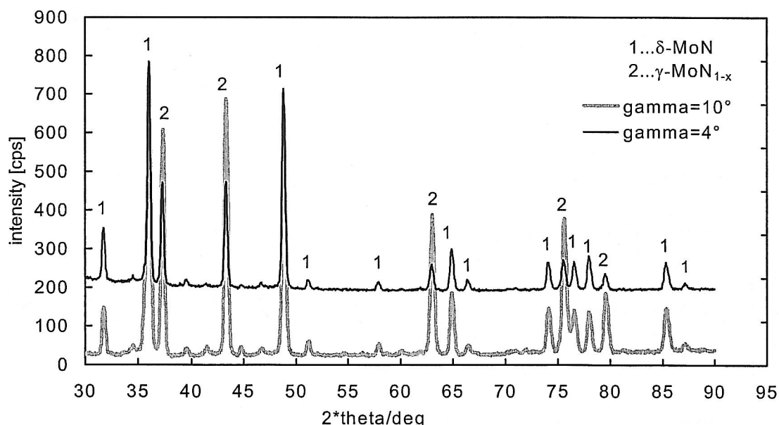
Fig. 3 GAXRD pattern of a nitrated Mo sheet; (900°C; 20l/h \text{NH}_3 ; 72h)
