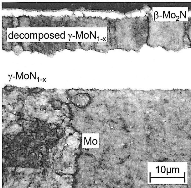
Fig. 4 Microstructure of the near surface area of a Mo-N diffusion couple; 1200°C, 10l/hNH 3 , 40h
