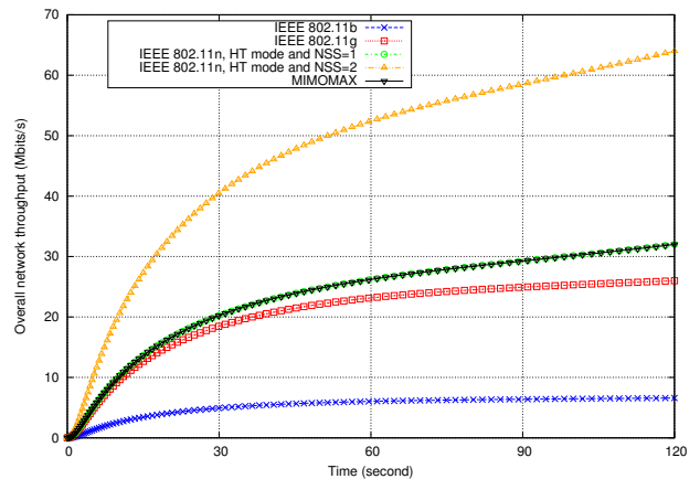
Fig. 7. Throughput of a single-hop wireless network.
