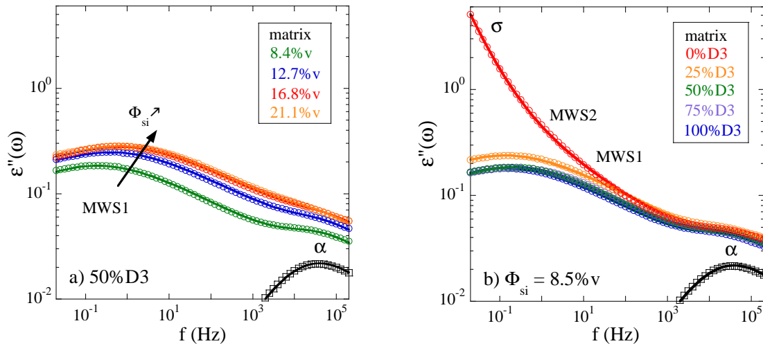
Figure 2: Dielectric loss spectra at T = 273 K for nanocomposites with a) different silica volume fractions ( \Phi_{si} = 8.4, 12.7, 16.8 and 21.1\% v from bottom to top, 50%D3), and b) different amounts of graftable chains (%D3 = 0, 25, 50, 75 and 100, from top to bottom, \Phi_{si} \approx 8.5\% v). The matrix signal is shown as black squares. Solid lines are fits to the experimental data by means of eq 1.
