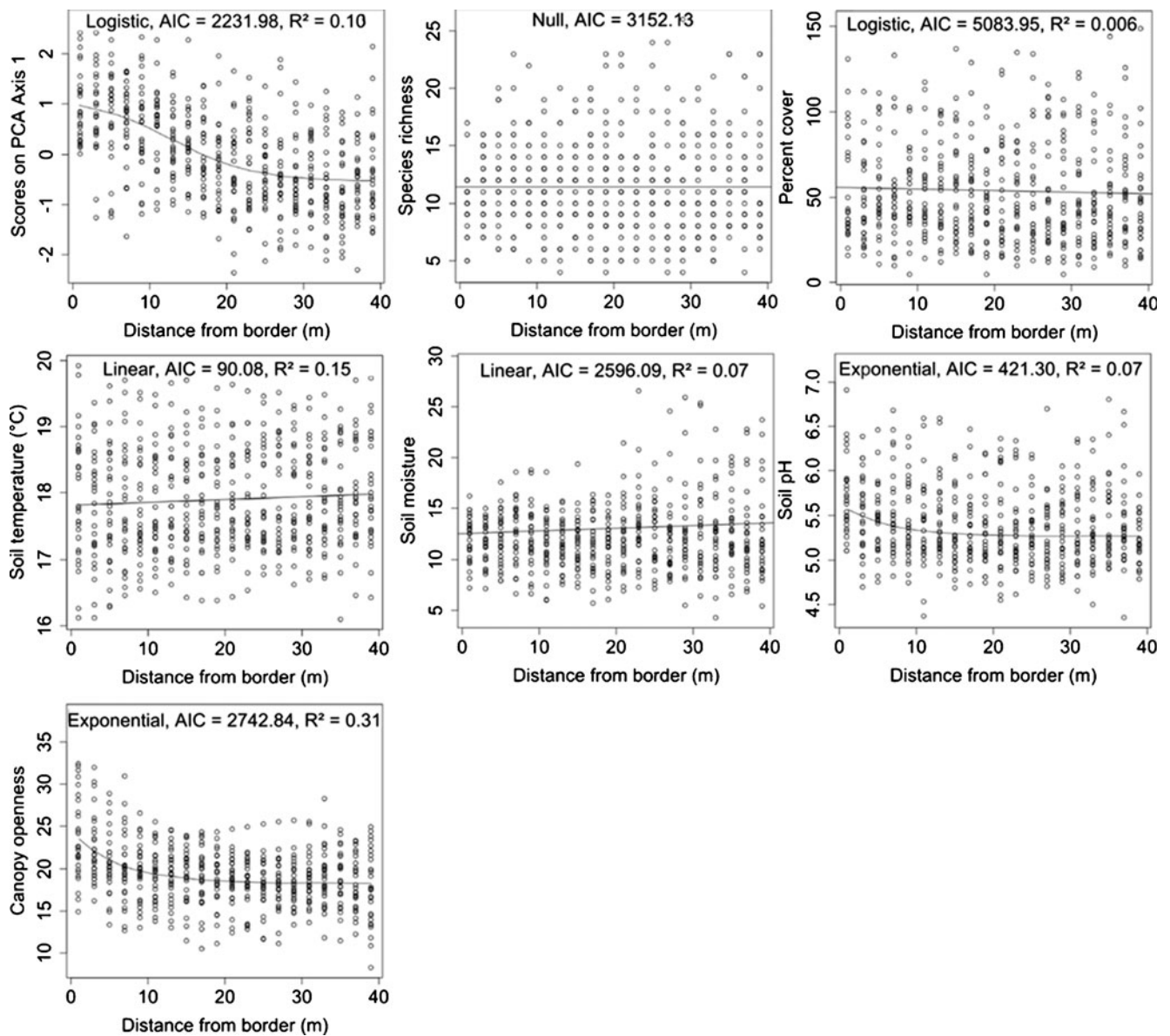
Fig. 1 Best model selected for each biotic and abiotic variable overall transects ( n=28 ). Models consisted in nonlinear mixed effects models with distance from the border, edge orientation, topography, adjacent land cover, and forest patch size as fixed terms and transect identity as random term
