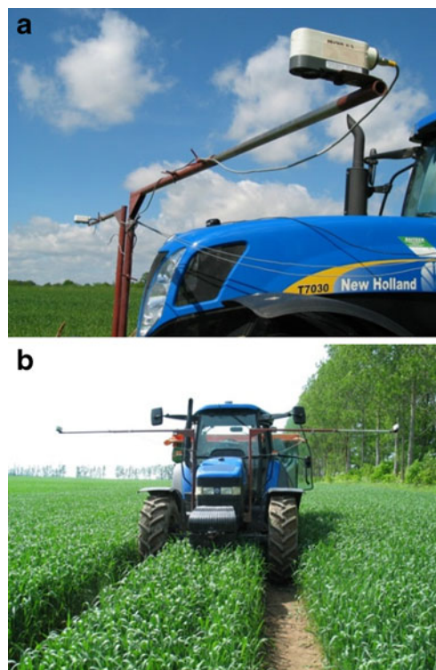
Fig. 2 a, b Active-light proximal sensors can be used to monitor wheat nitrogen status. These sensors could help farmers to plan variable nitrogen application rates. a This shows a particular of the system developed for using two Crop Circle™ (Holland Scientific, Lincoln, NE) sensors, while b shows an example of use of these sensors in a wheat crop in Poland (from Samborski S., Department of Agronomy, Faculty of Agriculture and Biology, Warsaw University of Life Sciences)
