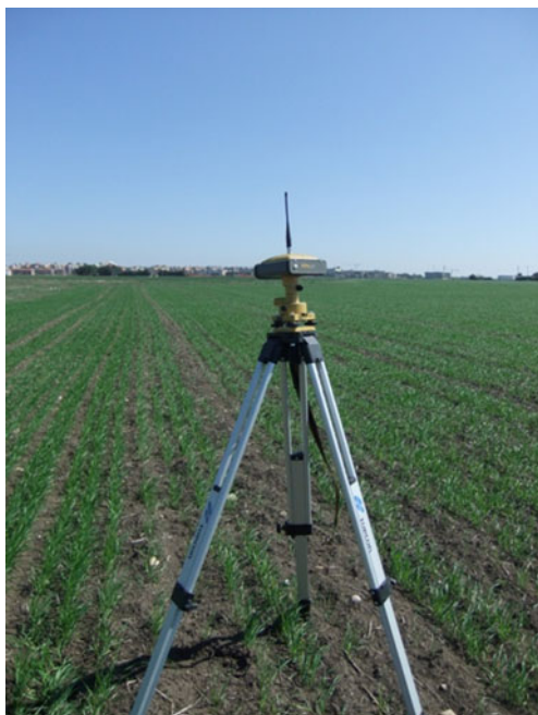
Fig. 1 Sampling location (point coordinates) and elevation can be recorded by using a differential global positioning system (DGPS, HiPer® 27 Pro, TOPCON). It enhances the quality of location data gathered using global positioning system (GPS) receiver. The figure shows base station of the instrument positioned in a wheat field
