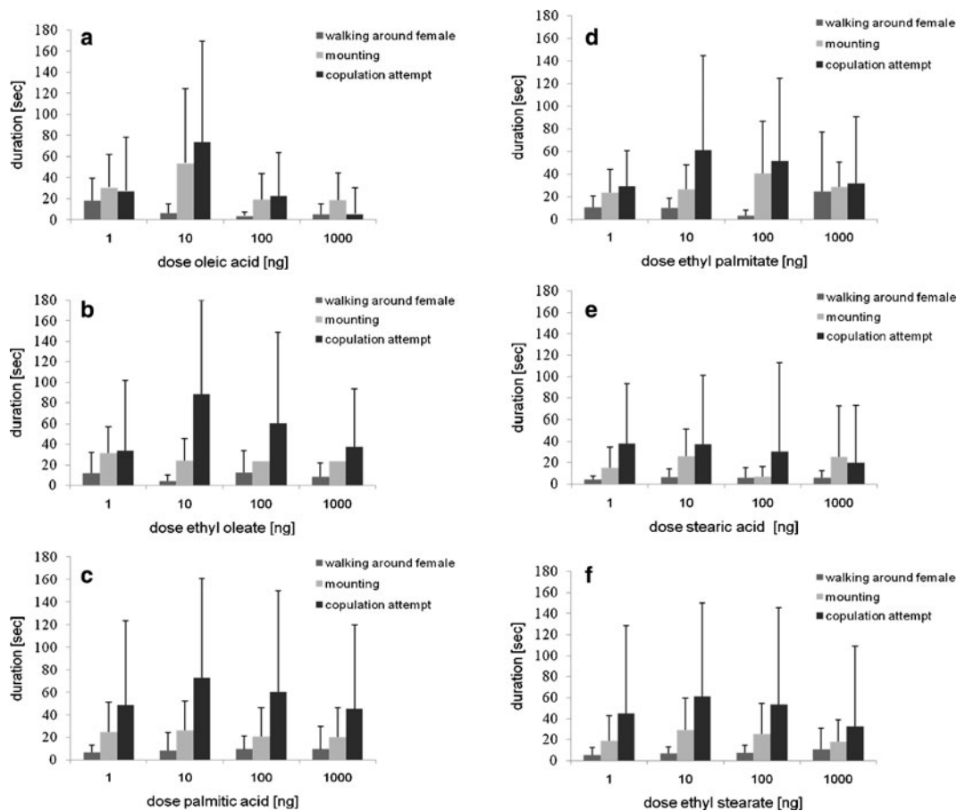
Figure 4. Response of males of V. destructor to a female deutochrysalis in the presence of single substances identified in the diethyl ether fraction of extracts of young females. Substances were dissolved in diethyl ether and applied in absolute amounts of 1, 10, 100, and 1,000 ng on filter paper.
