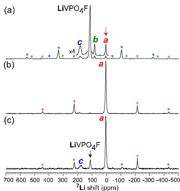
Figure 7. Selective excitation of ^7\text{Li} spins associated with defect environment 'a' in phase-pure \text{LiVPO}_4\text{F} (sample A) and subsequent through-space transfer of magnetization by fp-RFDR to its dipole-dipole-coupled ^7\text{Li} spins. (a) Solid-state ^7\text{Li} spin-echo MAS NMR spectrum (identical to Figure 4a). Site-selective ^7\text{Li} fp-RFDR NMR spectra acquired with (b) 0 and (c) 10 ms mixing times. Asterisks indicate spinning sidebands and are color coded to correspond to the different lithium environments.
