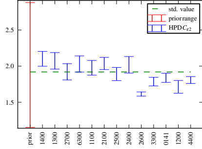
(a) C_{\epsilon 2} of the k - \epsilon model.
