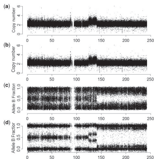
Fig. 1. TCNs (panels a and b) and BAFs (panels c and d) in Chr. 2 from ovarian tumor TCGA-23-1027 before CalMaTe (panels a and c) and after CalMaTe (panels b and d) based on Affymetrix GenomeWideSNP_6 data. Ditto for Illumina Human1M-Duo data is in Figure S4
