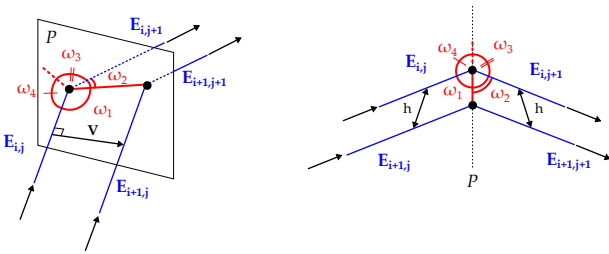
Figure 3: Generation of a discrete Monge surface by edge offset: perspective (left) and top view (right).
