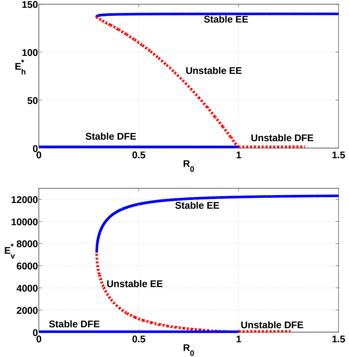
Figure 2: The backward bifurcation curves for model system (15) in the (\mathcal{R}_0, E_h^*) , and (\mathcal{R}_0, E_v^*) planes. The parameter \beta_{hv} is varied in the range [0, 0.2810] to allow \mathcal{R}_0 to vary in the range [0, 1.5] . Two endemic equilibrium points coexist for values of \mathcal{R}_0 in the range (0.2894, 1) (corresponding to the range (0.0105, 0.1249) of \beta_{hv} ). The notation EE and DFE stand for endemic equilibrium and disease-free equilibrium, respectively. Solid line represent stable equilibria and dash line stands for unstable equilibria.
