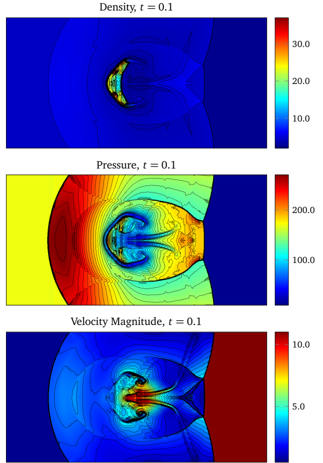
Figure 14. Cloud-Shock Interaction. Contour plots of the density (top), pressure (middle), and velocity magnitude (bottom) at time t = 0.1 . The computations were done with a RKFDV with WENO7 reconstruction. The computational domain is the box [0, 2] \times [0, 1] , discretized by using a mesh of 800 \times 400 cells.
