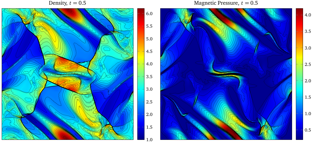
Figure 9. Orszag-Tang vortex problem. Contour plots of the density (left) and the magnetic pressure (right) at time t = 0.5 . Computations were done with a RK4V method with WENO7 reconstruction. The computational domain is the box [0, 1] \times [0, 1] , discretized by using a mesh of 600 \times 600 cells.
