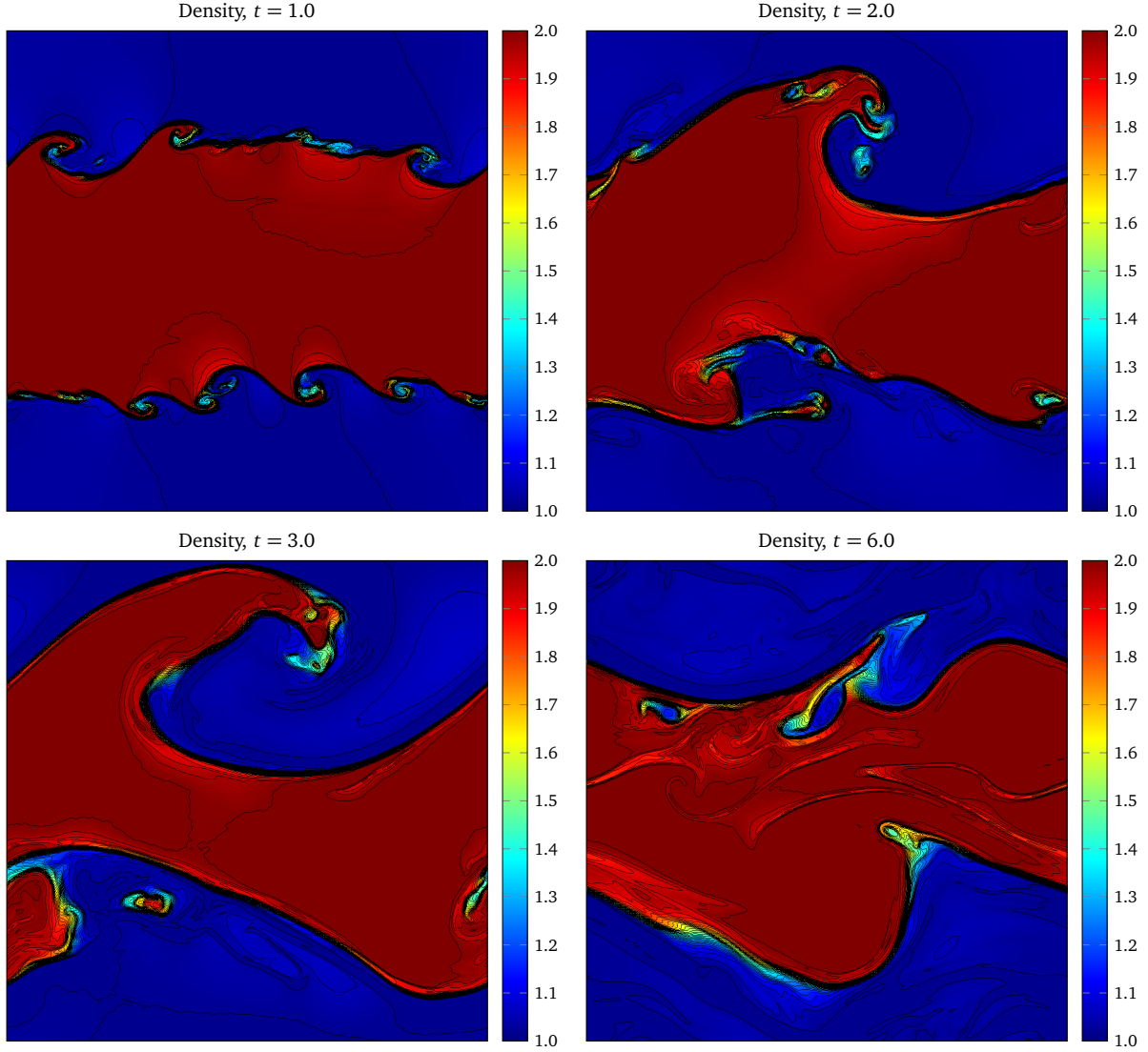
Figure 15. Kelvin-Helmholtz instability. From left to right and from top to bottom, contour plots of the density at simulation times t \in \{1.0, 2.0, 3.0, 6.0\} . The solution was computed with a RK-FV-WENO7 scheme on a mesh made of 600 \times 600 cells.
