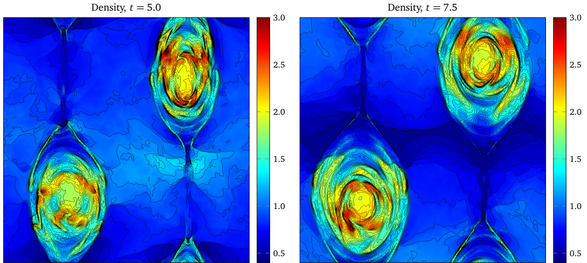
Figure 8. Current sheet problem. Contour plots of the density at times t = 5.0 (left) and t = 7.5 (right). The calculations were performed with a RKFD with WENO7 reconstruction. The computational domain is the box [-0.5, +0.5] \times [-0.5, +0.5] , discretized by using a mesh of 600 \times 600 cells.
