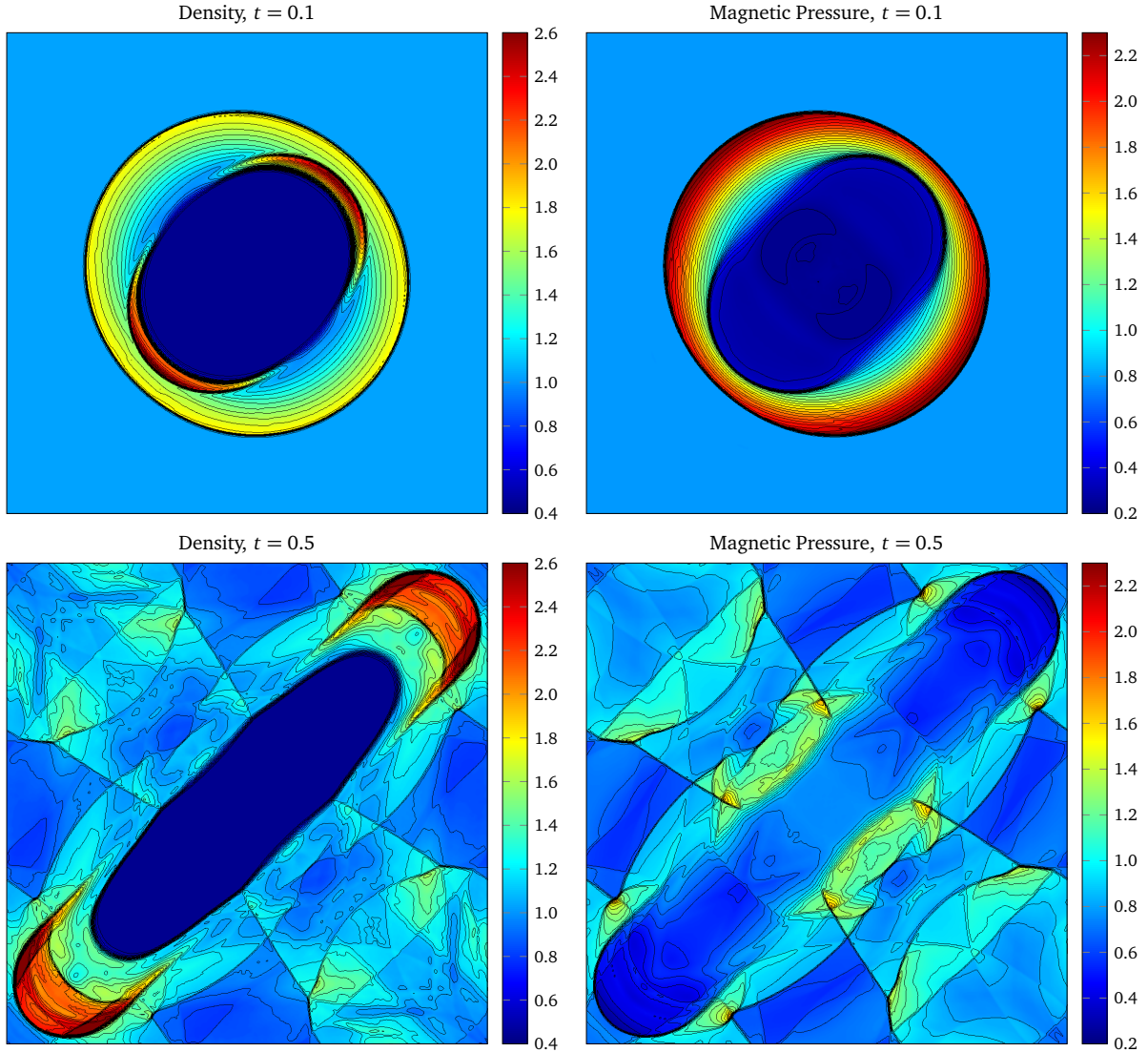
Figure 11. Cylindrical blast wave. Contour plots of the density (left) and magnetic pressure (right) at times t = 0.10 (top) and t = 0.50 (bottom) obtained with a finite volume method with WENO7 reconstruction. The computational domain is the box [0, 1] \times [0, 1] , discretized by using a mesh of 600 \times 600 cells.
