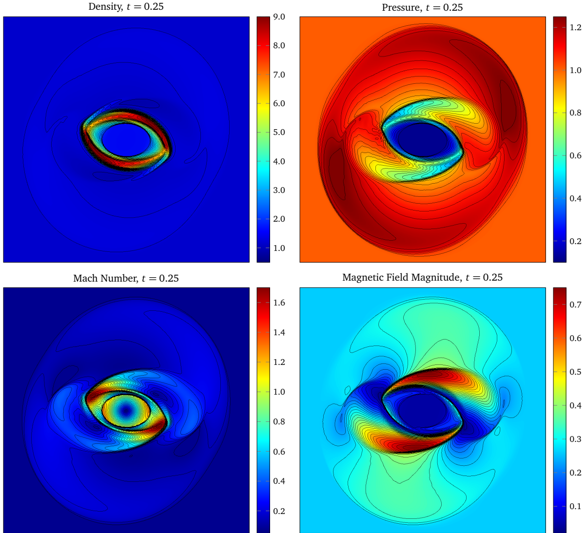
Figure 12. Rotor problem. Contour plots of the density, pressure, Mach number, and the magnitude of the magnetic field at time t = 0.25 . These calculations were performed with a RK4V with hybrid WENO7/WENO3 reconstruction. The computational domain is the box [0, 1] \times [0, 1] , discretized by using a mesh of 600 \times 600 cells.
