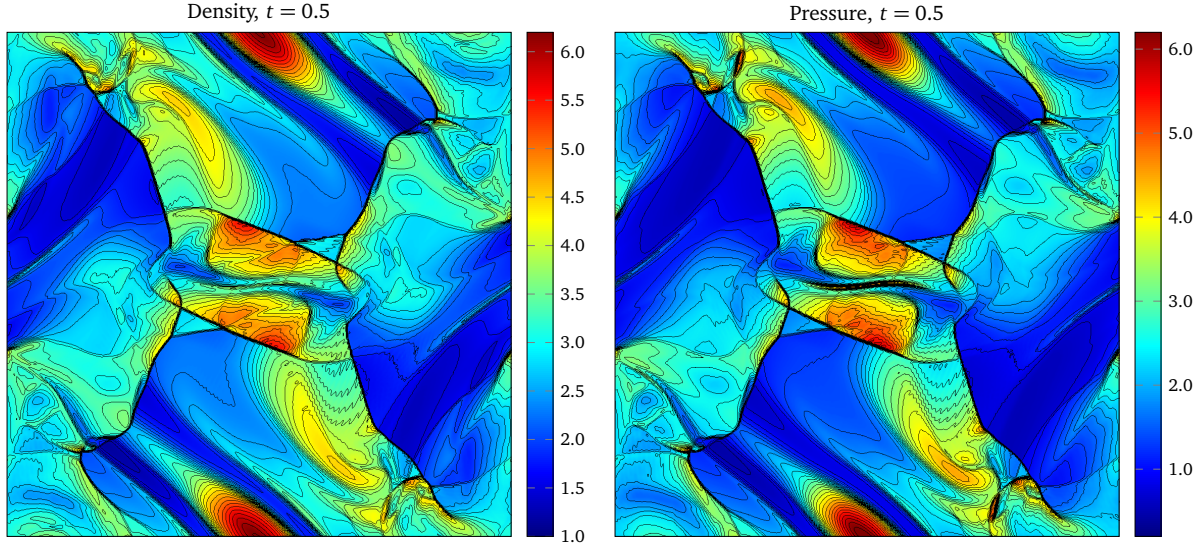
Figure 9. Orszag-Tang vortex problem. Contour plots of the density (left) and the pressure (right) at time t = 0.5 . Computations were done with a RKFV method with WENO7 reconstruction. The computational domain is the box [0, 1] \times [0, 1] , discretized by using a mesh of 600 \times 600 cells.
