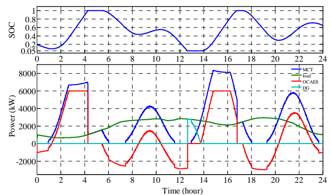
Fig. 12 Simulation results (SOC and power) when the tide speed amplitude is increased by 10%
